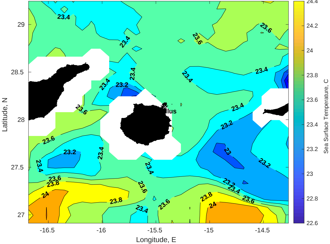
SST for Nautilus at 06-Nov-2025 00:00:00
