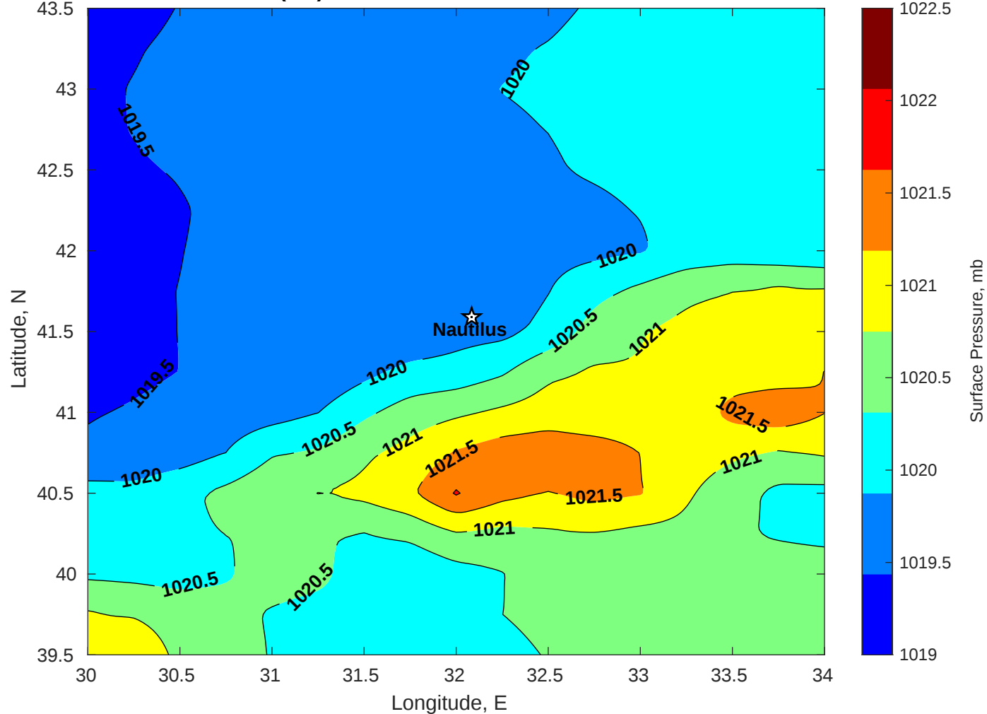
Surface Pressure (mb) for Nautilus at 09-Nov-2025 00:00:00
