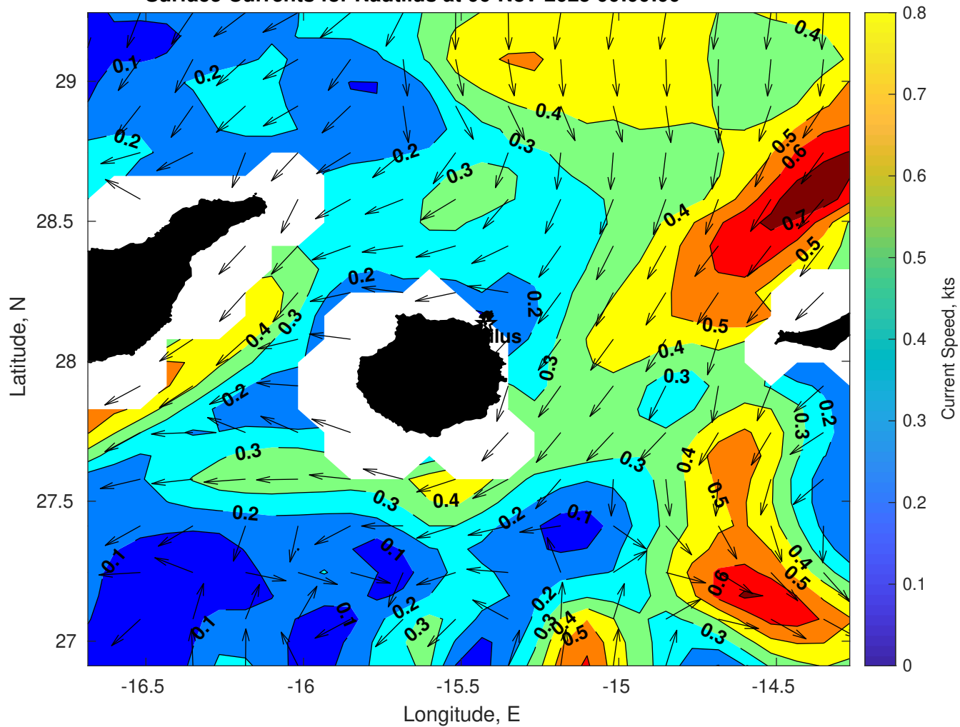
Surface Currents for Nautilus at 06-Nov-2025 00:00:00
