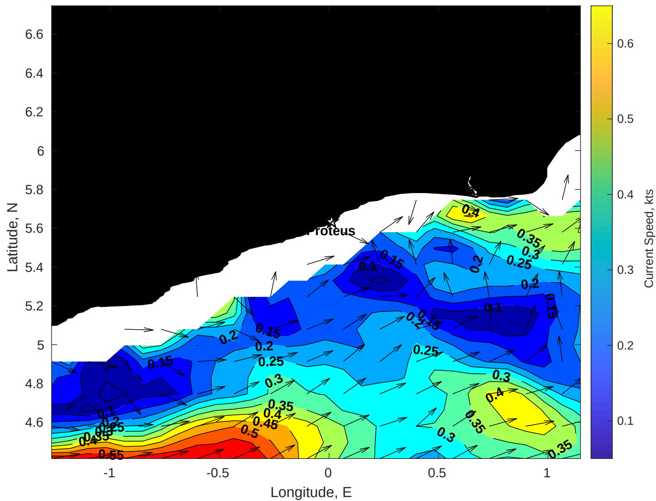
Surface Currents for Proteus at 06-Nov-2025 00:00:00
