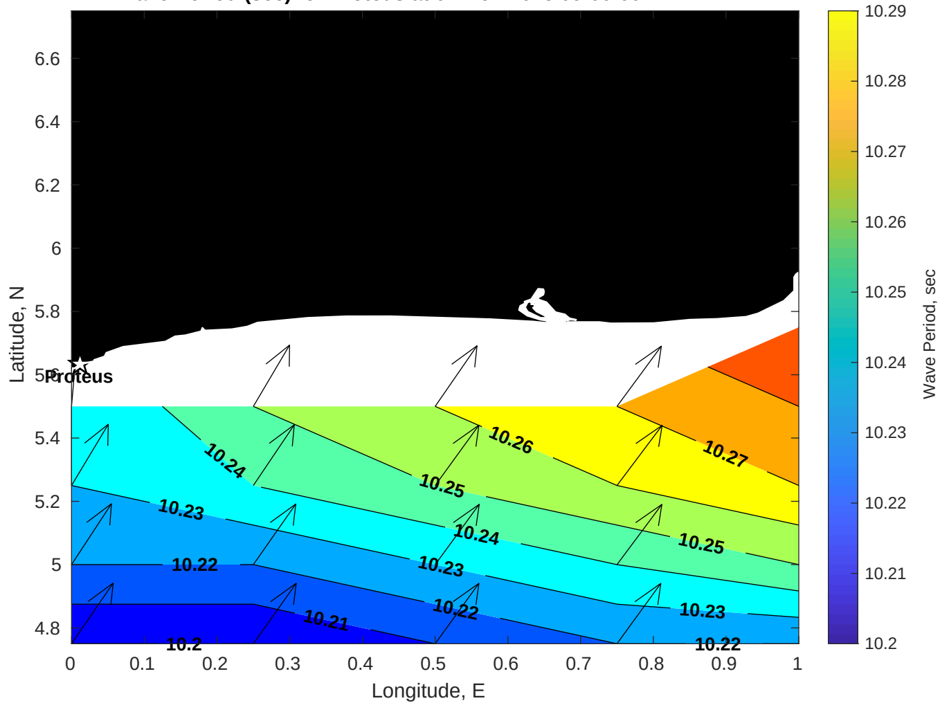
Wave Period (sec) for Proteus at 07-Nov-2025 09:00:00
