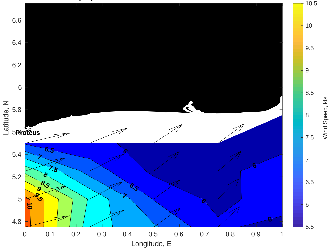
Winds (kts) for Proteus at 07-Nov-2025 09:00:00
