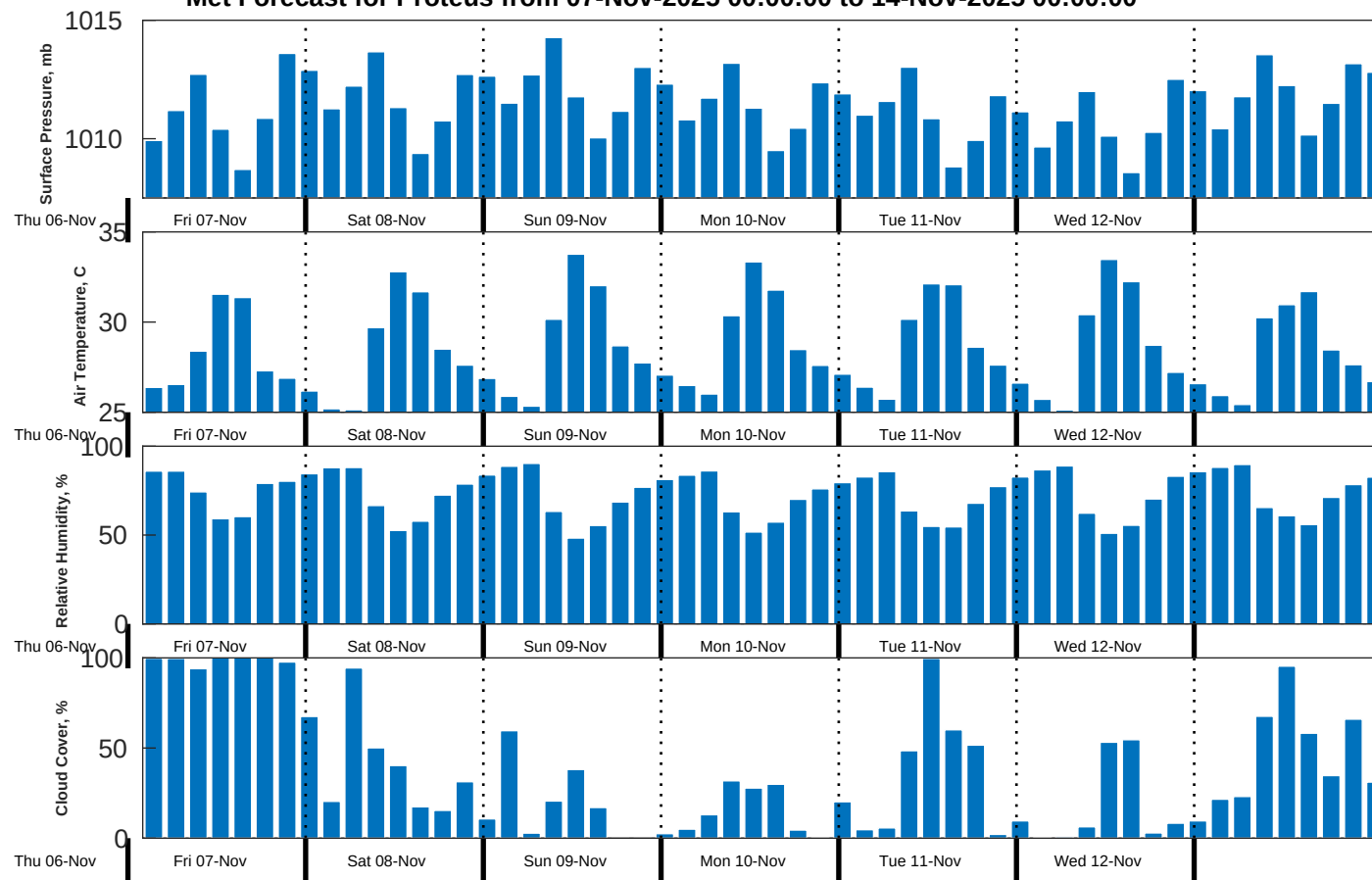
Met Forecast for Proteus from 07-Nov-2025 00:00:00 to 14-Nov-2025 00:00:00
