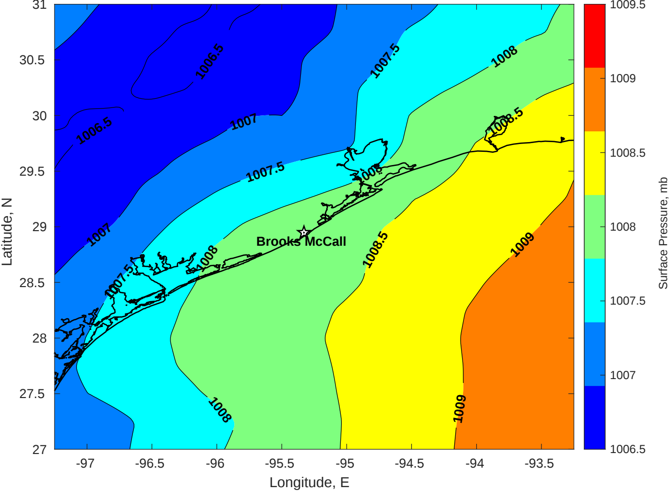
Surface Pressure (mb) for Brooks McCall at 08-Nov-2025 00:00:00
