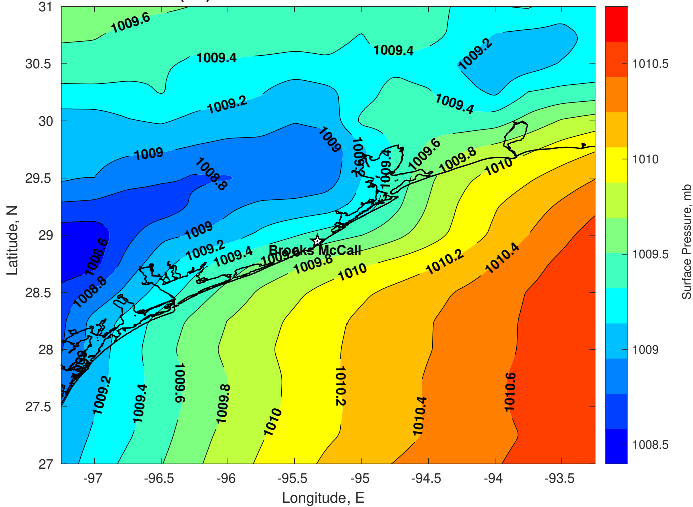
Surface Pressure (mb) for Brooks McCall at 09-Nov-2025 00:00:00
