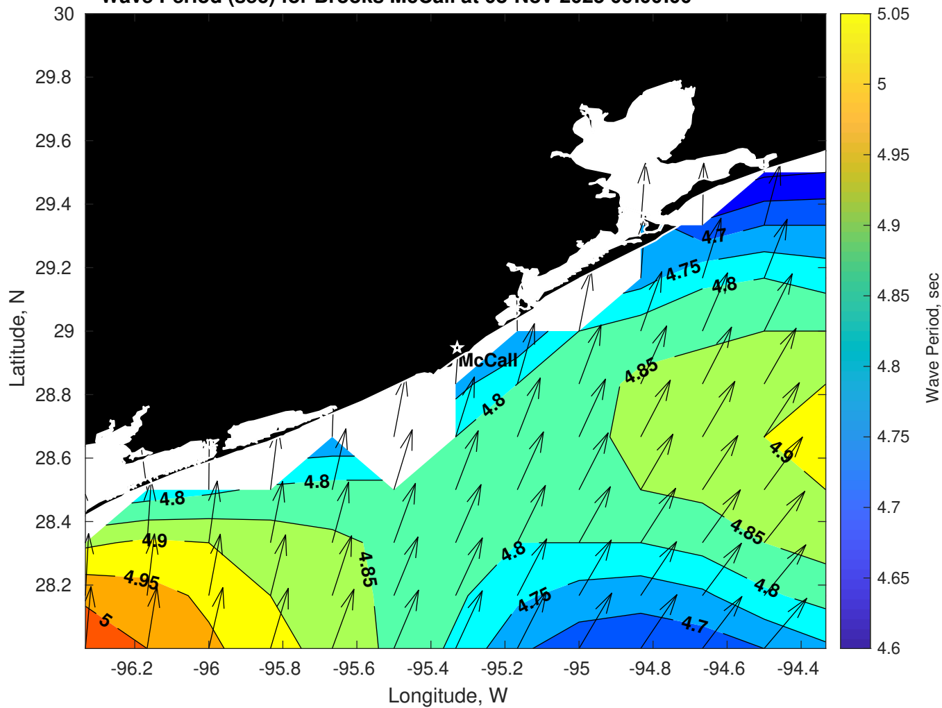
Wave Period (sec) for Brooks McCall at 08-Nov-2025 09:00:00
