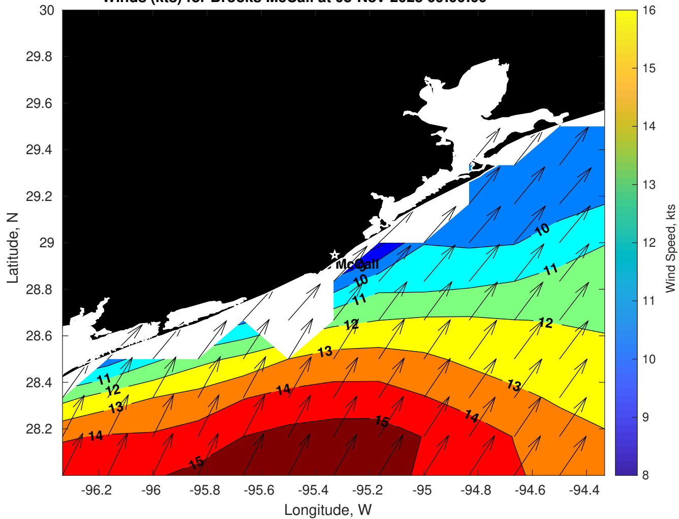
Winds (kts) for Brooks McCall at 08-Nov-2025 09:00:00
