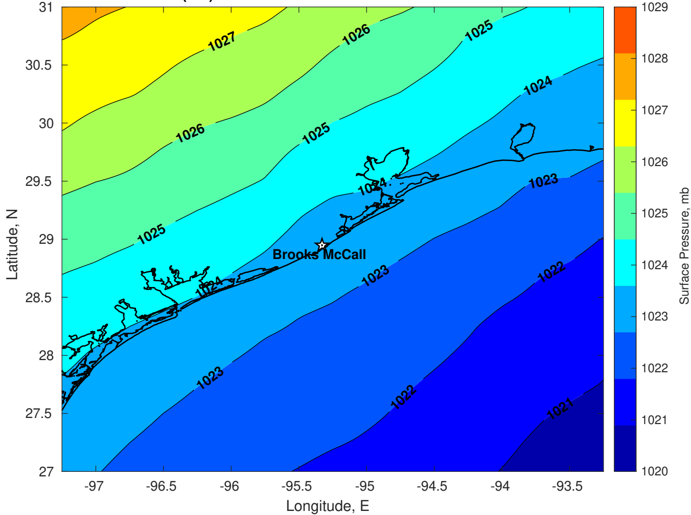
Surface Pressure (mb) for Brooks McCall at 10-Nov-2025 00:00:00
