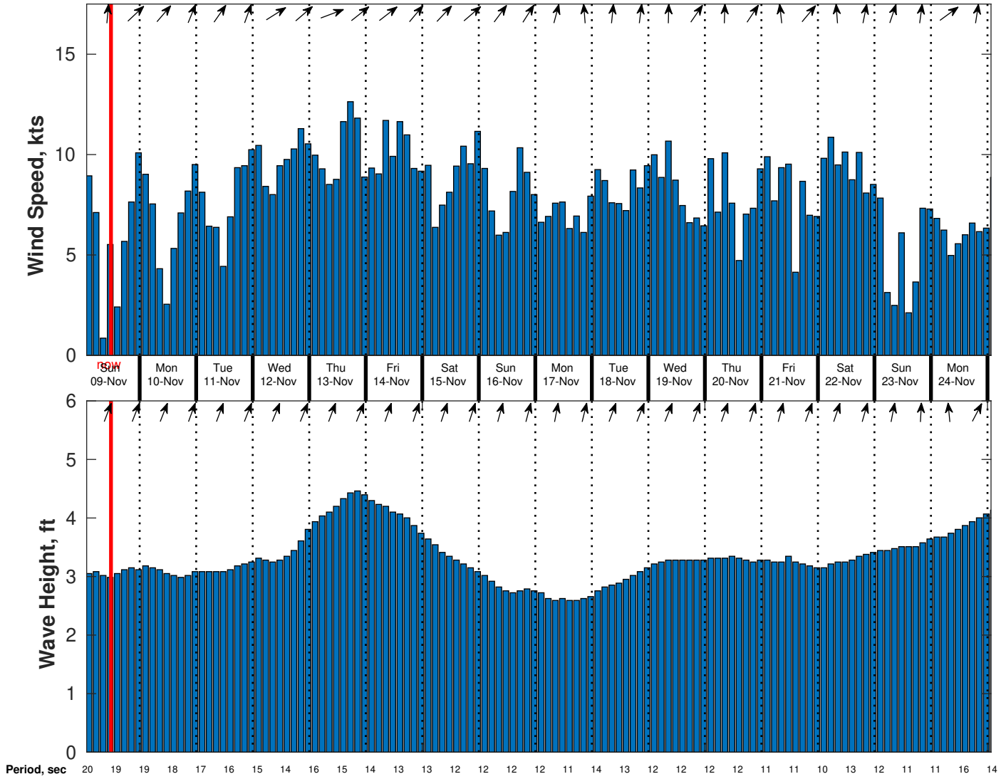
Wind & Wave Forecast for CSA (ONHYM) PPL EBS - Cote d'Ivoire from 08-Nov-2025 01:00:00 to 24-Nov-2025 01:00:00
