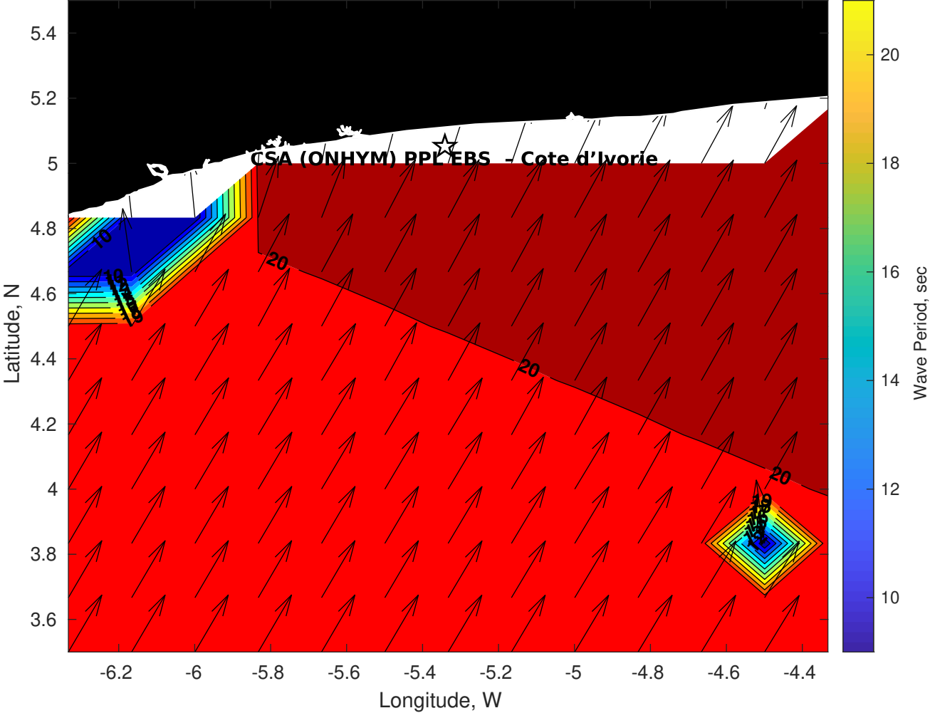
Wave Period (sec) for CSA (ONHYM) PPL EBS - Cote d'Ivoire at 08-Nov-2025 09:00:00
