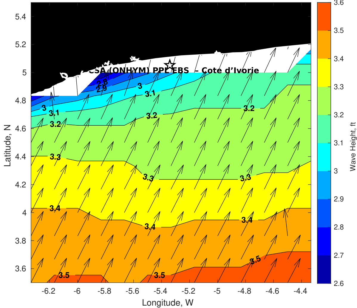
Wave Height (ft) for CSA (ONHYM) PPL EBS - Cote d'Ivoire at 08-Nov-2025 09:00:00
