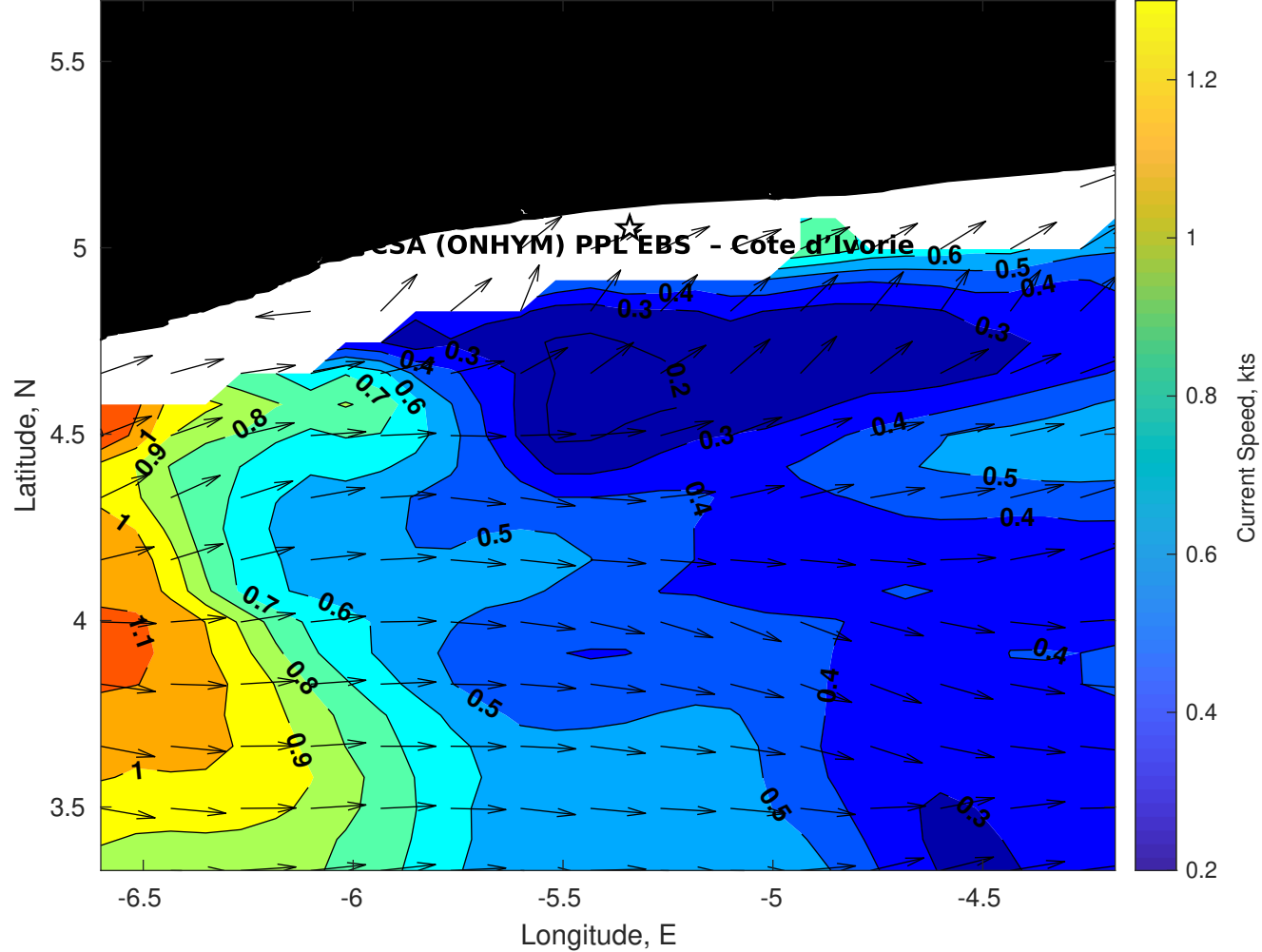
Surface Currents for CSA (ONHYM) PPL EBS - Cote d'Ivoire at 07-Nov-2025 00:00:00
