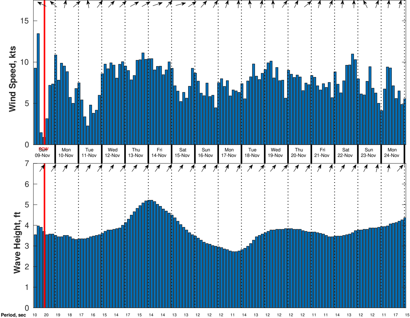
Wind & Wave Forecast for CSA (ONHYM) PPL EBS - Ghana from 08-Nov-2025 02:00:00 to 24-Nov-2025 02:00:00
