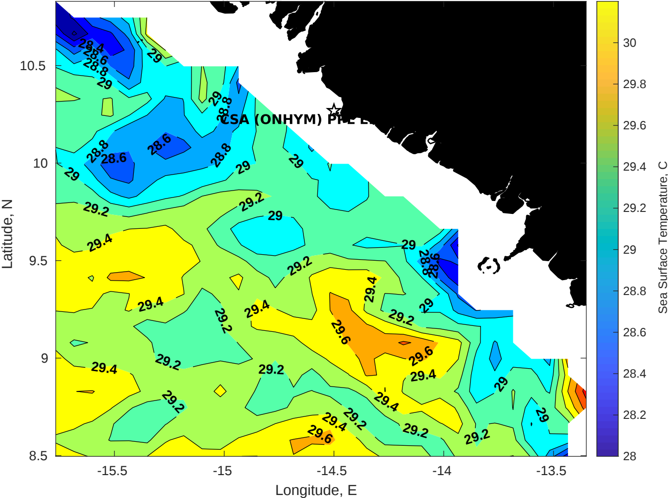
SST for CSA (ONHYM) PPL EBS - Guinea at 07-Nov-2025 00:00:00
