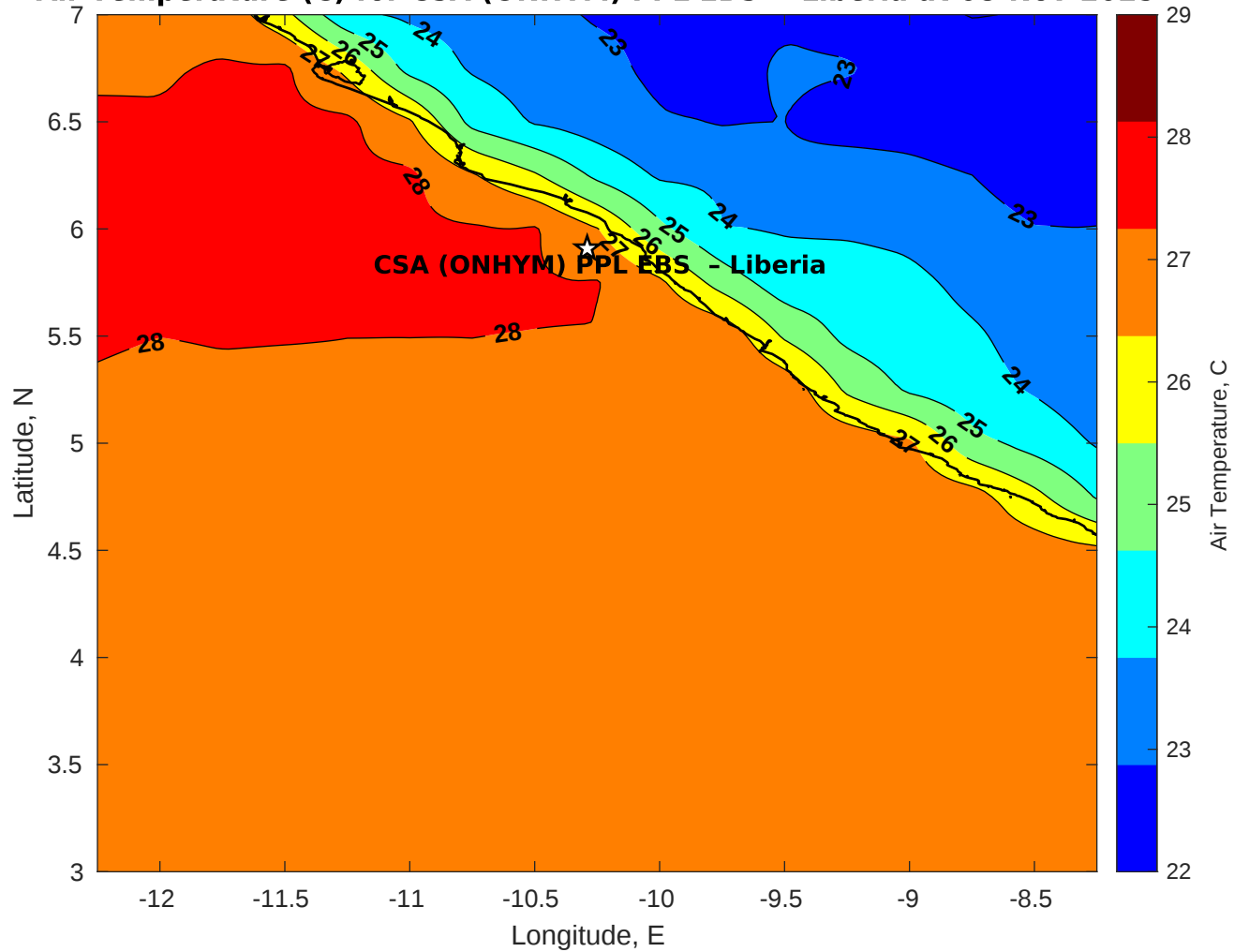
Air Temperature (C) for CSA (ONHYM) PPL EBS - Liberia at 08-Nov-2025
