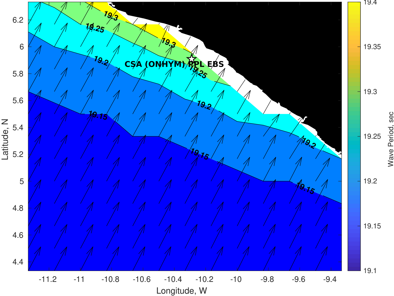
Wave Period (sec) for CSA (ONHYM) PPL EBS - Liberia at 08-Nov-2025 09:00:00
