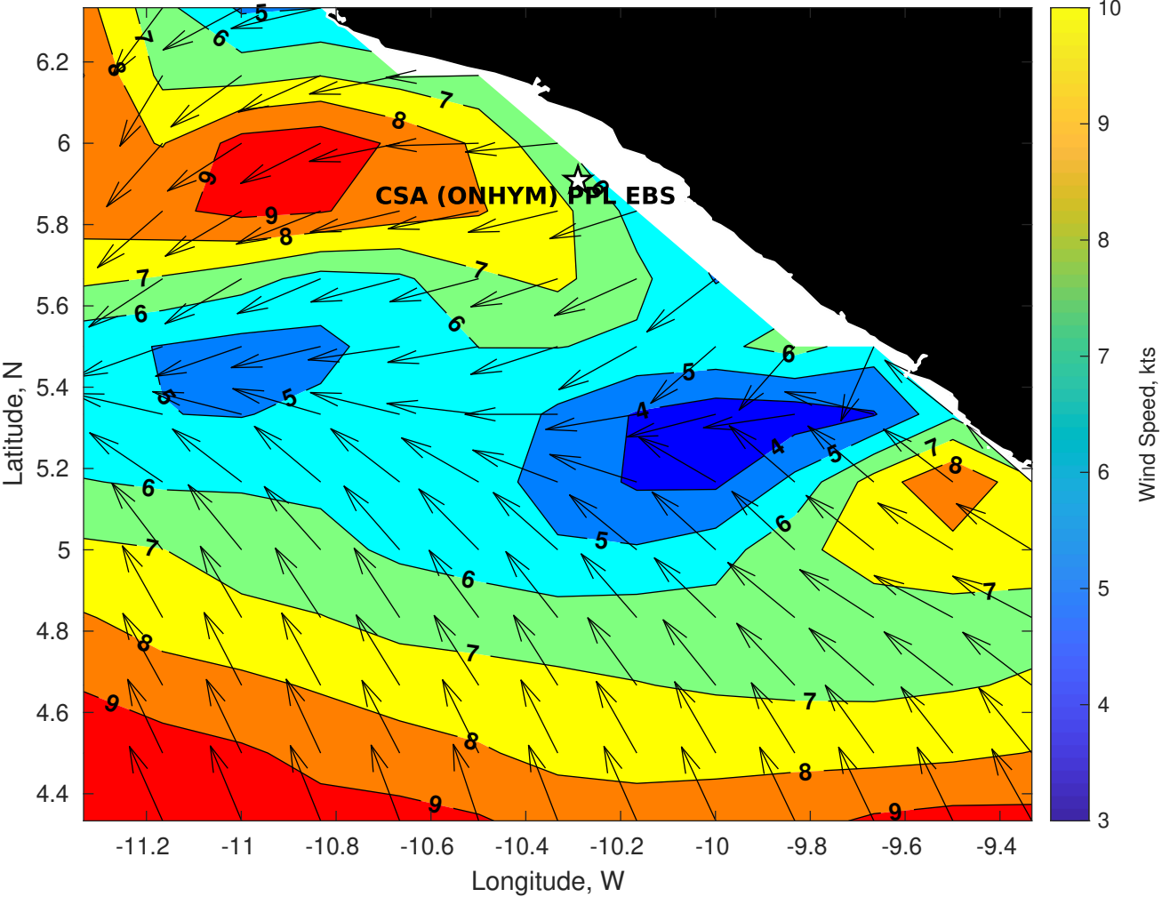
Winds (kts) for CSA (ONHYM) PPL EBS - Liberia at 08-Nov-2025 09:00:00
