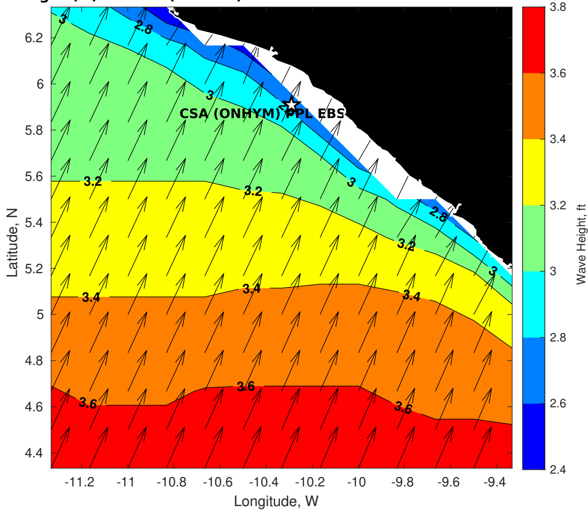
Wave Height (ft) for CSA (ONHYM) PPL EBS - Liberia at 08-Nov-2025 09:00:00
