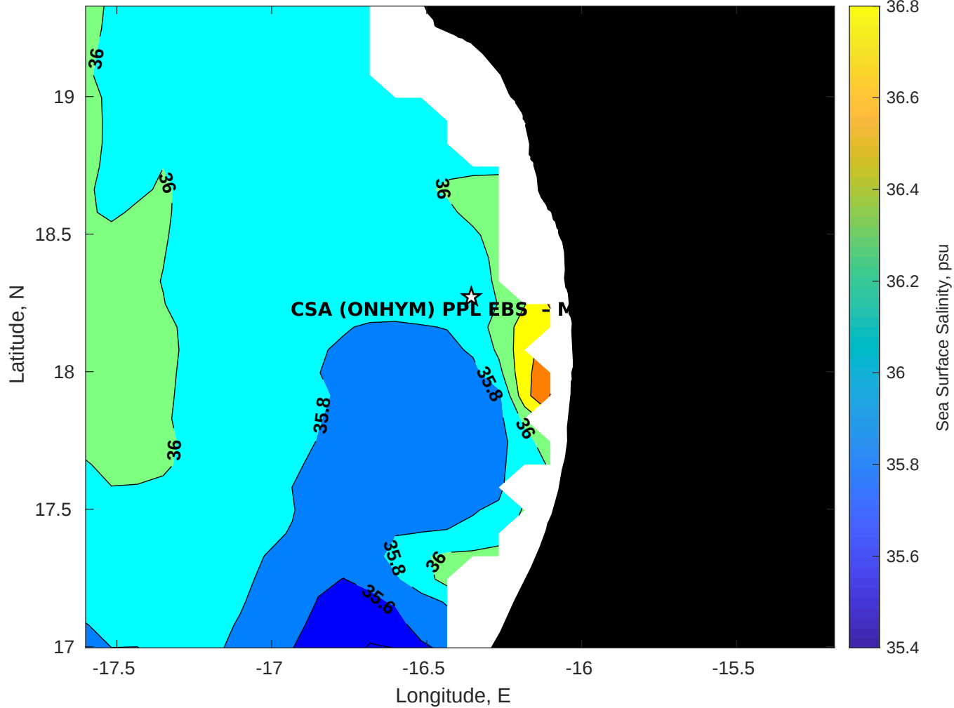
Surface Salinity for CSA (ONHYM) PPL EBS - Mauritania at 07-Nov-2025 00:00:00
