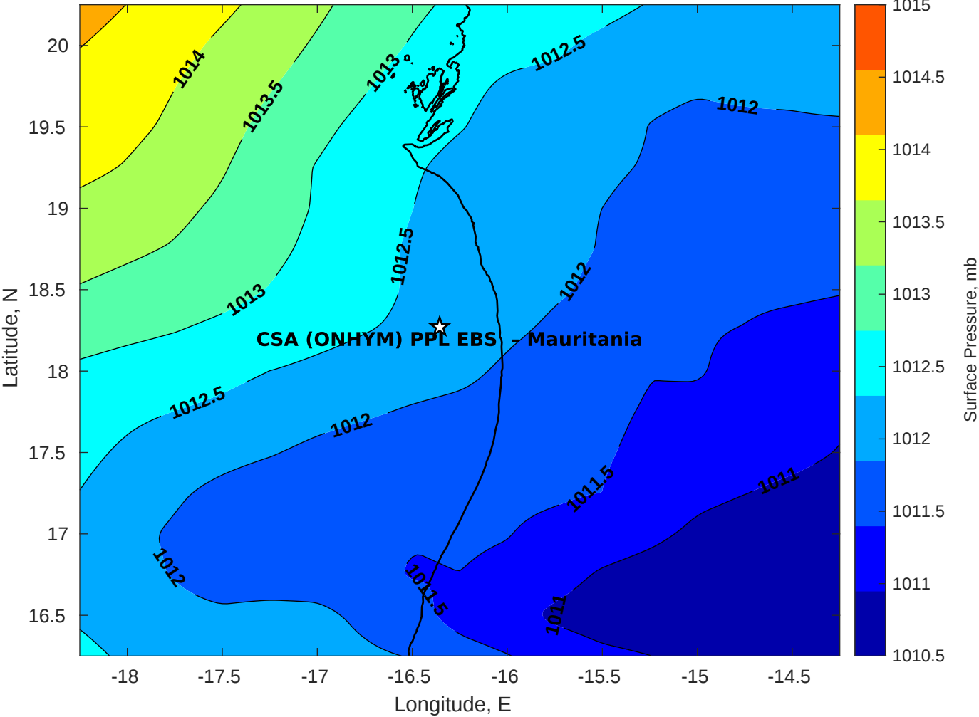
Surface Pressure (mb) for CSA (ONHYM) PPL EBS - Mauritania at 08-Nov-2025 00:00:00
