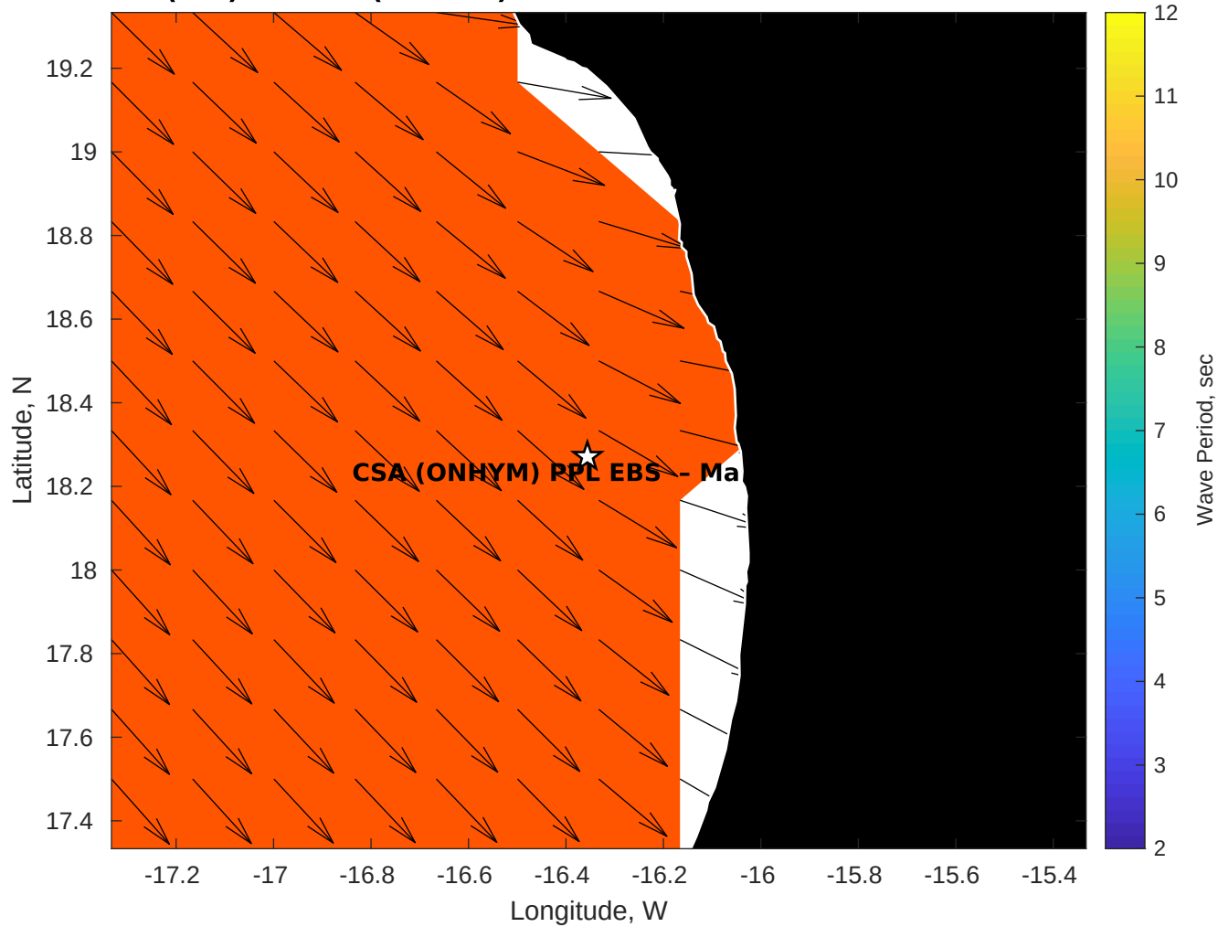
Wave Period (sec) for CSA (ONHYM) PPL EBS - Mauritania at 08-Nov-2025 09:00:00
