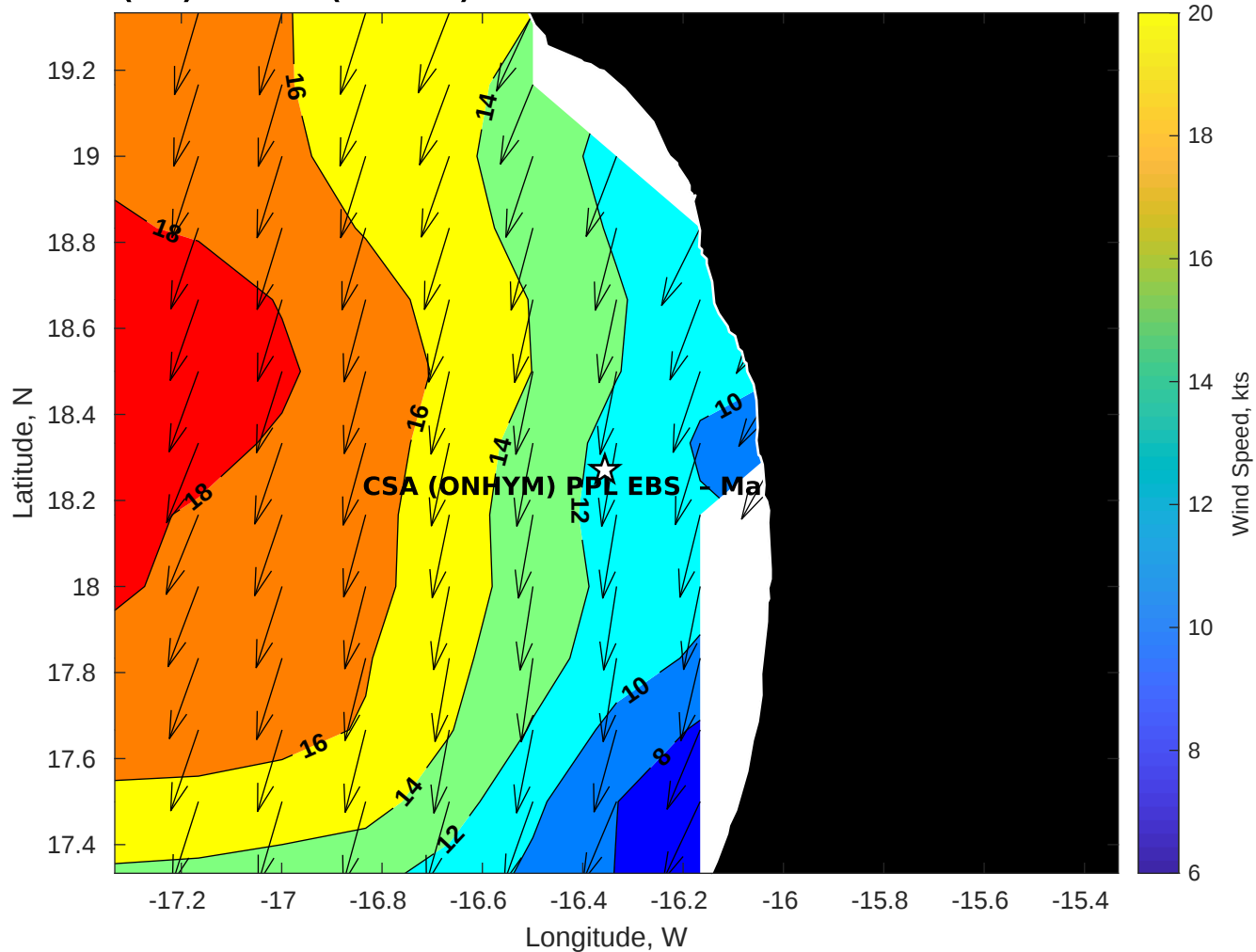
Winds (kts) for CSA (ONHYM) PPL EBS - Mauritania at 08-Nov-2025 09:00:00
