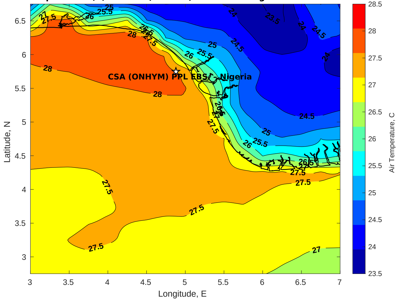
Air Temperature (C) for CSA (ONHYM) PPL EBS - Nigeria at 08-Nov-2025
