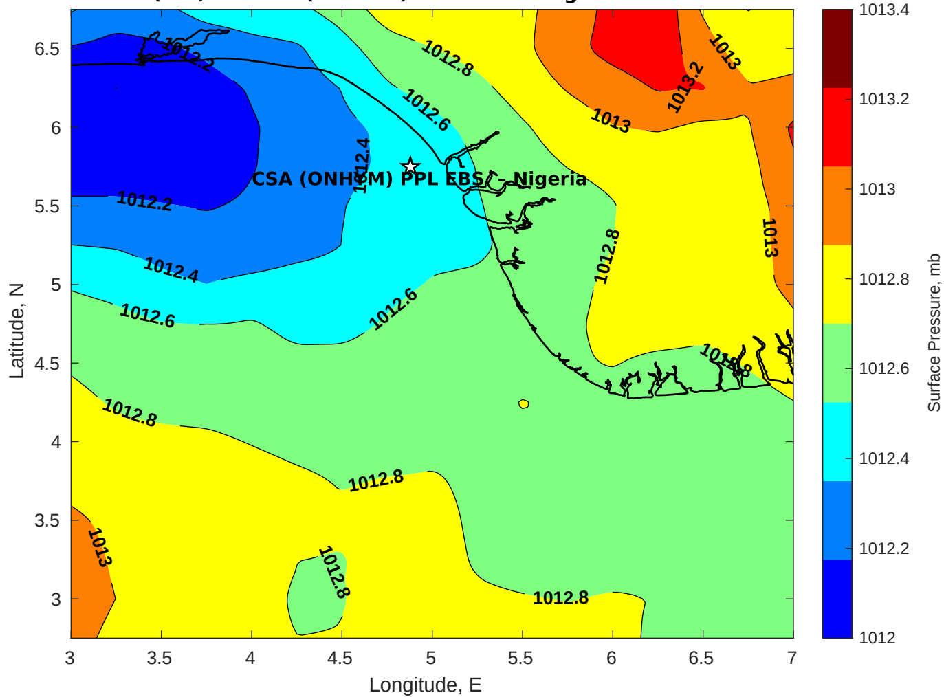
Surface Pressure (mb) for CSA (ONHYM) PPL EBS - Nigeria at 10-Nov-2025 00:00:00
