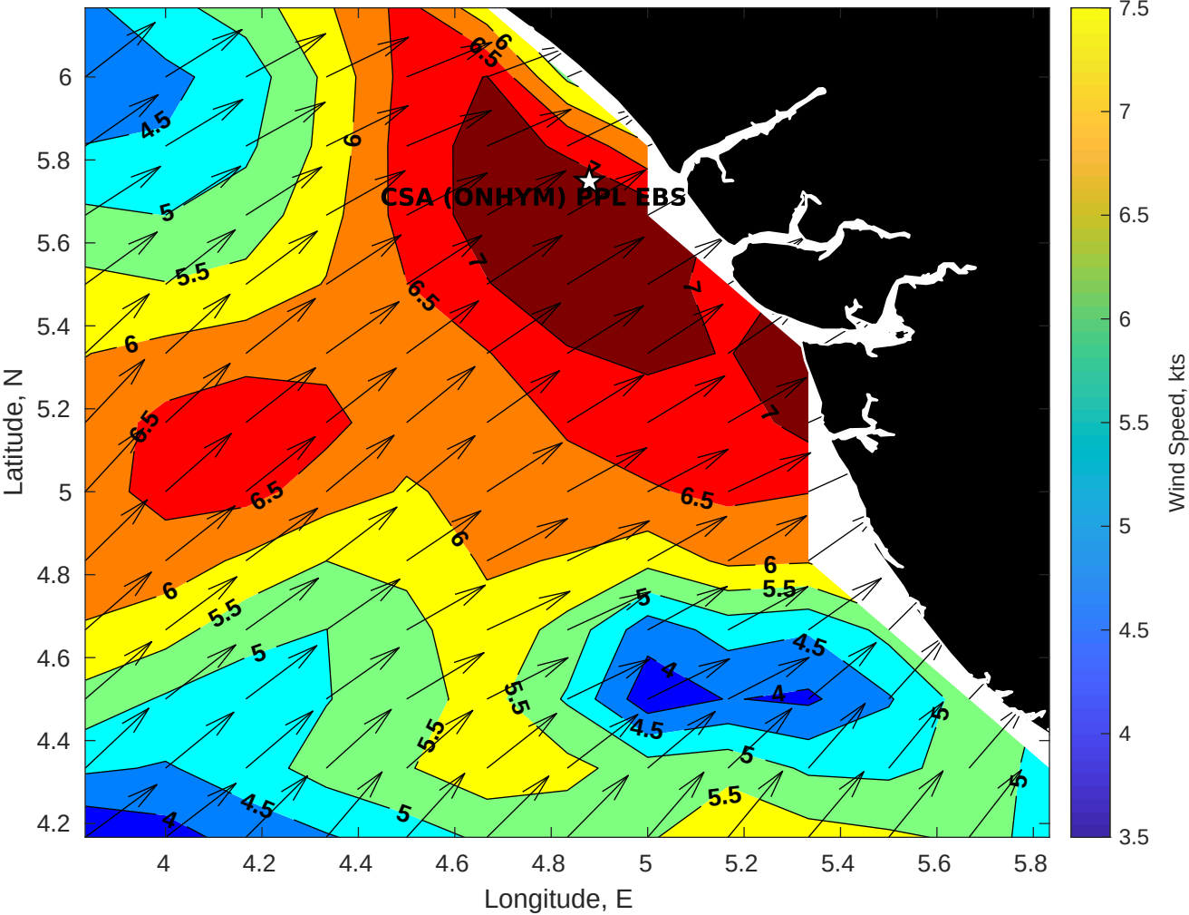
Winds (kts) for CSA (ONHYM) PPL EBS - Nigeria at 08-Nov-2025 09:00:00
