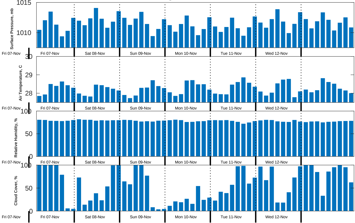
Met Forecast for CSA (ONHYM) PPL EBS - Nigeria from 08-Nov-2025 00:00:00 to 15-Nov-2025 00:00:00
