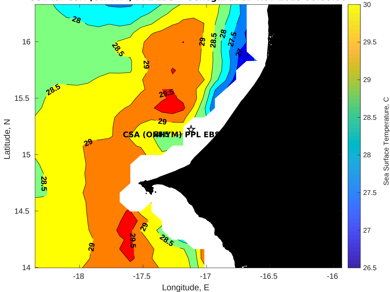
SST for CSA (ONHYM) PPL EBS - Senegal at 07-Nov-2025 00:00:00
