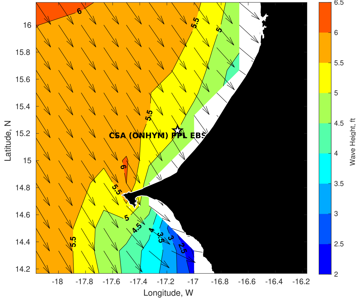
Wave Height (ft) for CSA (ONHYM) PPL EBS - Senegal at 08-Nov-2025 09:00:00
