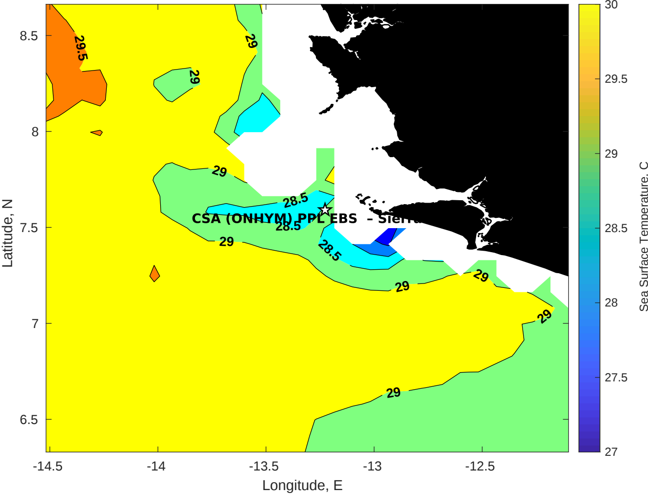
SST for CSA (ONHYM) PPL EBS - Sierra Leone at 07-Nov-2025 00:00:00
