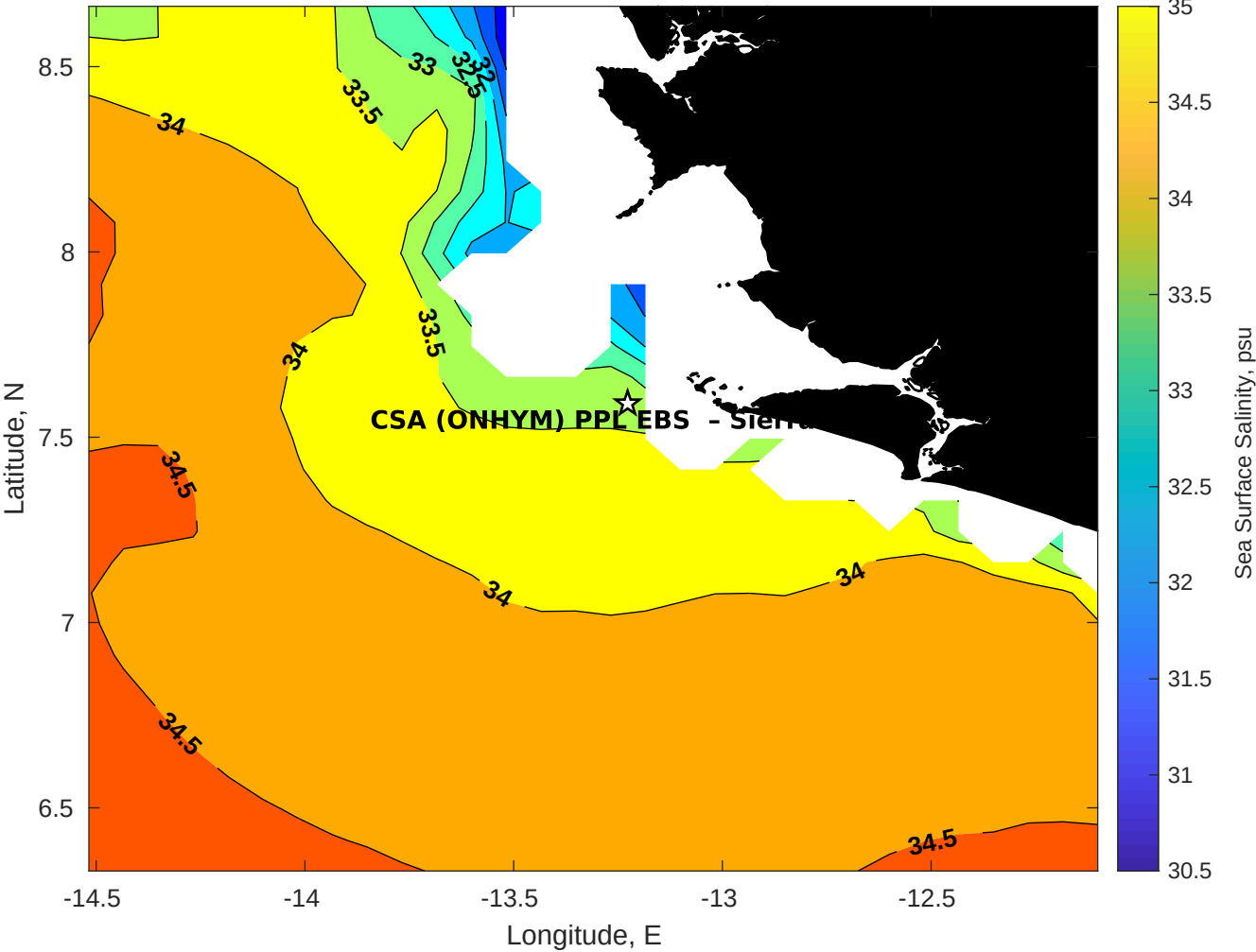
Surface Salinity for CSA (ONHYM) PPL EBS - Sierra Leone at 07-Nov-2025 00:00:00
