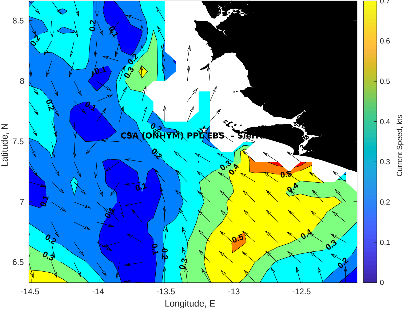
Surface Currents for CSA (ONHYM) PPL EBS - Sierra Leone at 07-Nov-2025 00:00:00
