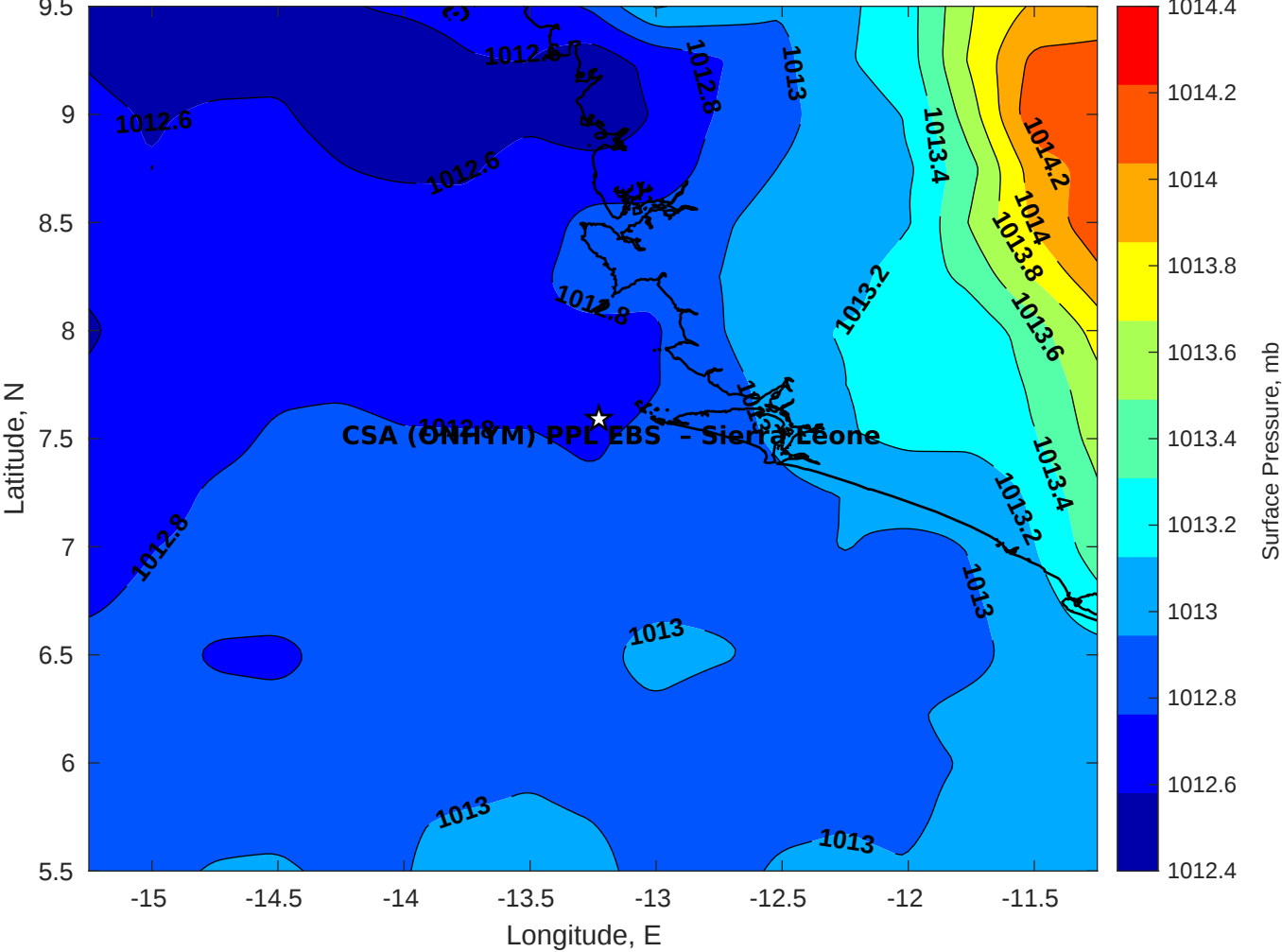
Surface Pressure (mb) for CSA (ONHYM) PPL EBS - Sierra Leone at 08-Nov-2025 00:00:00
