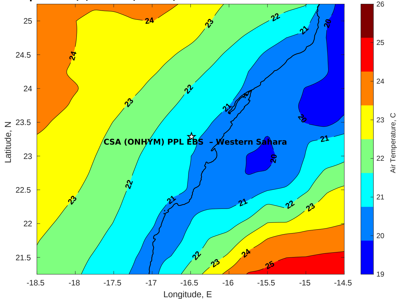
Air Temperature (C) for CSA (ONHYM) PPL EBS - Western Sahara at 08-Nov-2025
