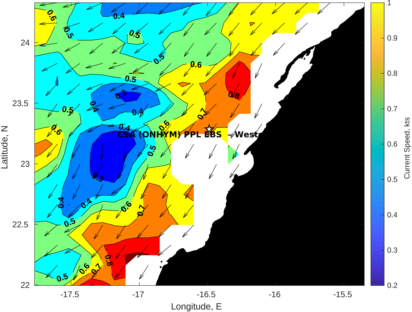
Surface Currents for CSA (ONHYM) PPL EBS - Western Sahara at 07-Nov-2025 00:00:00
