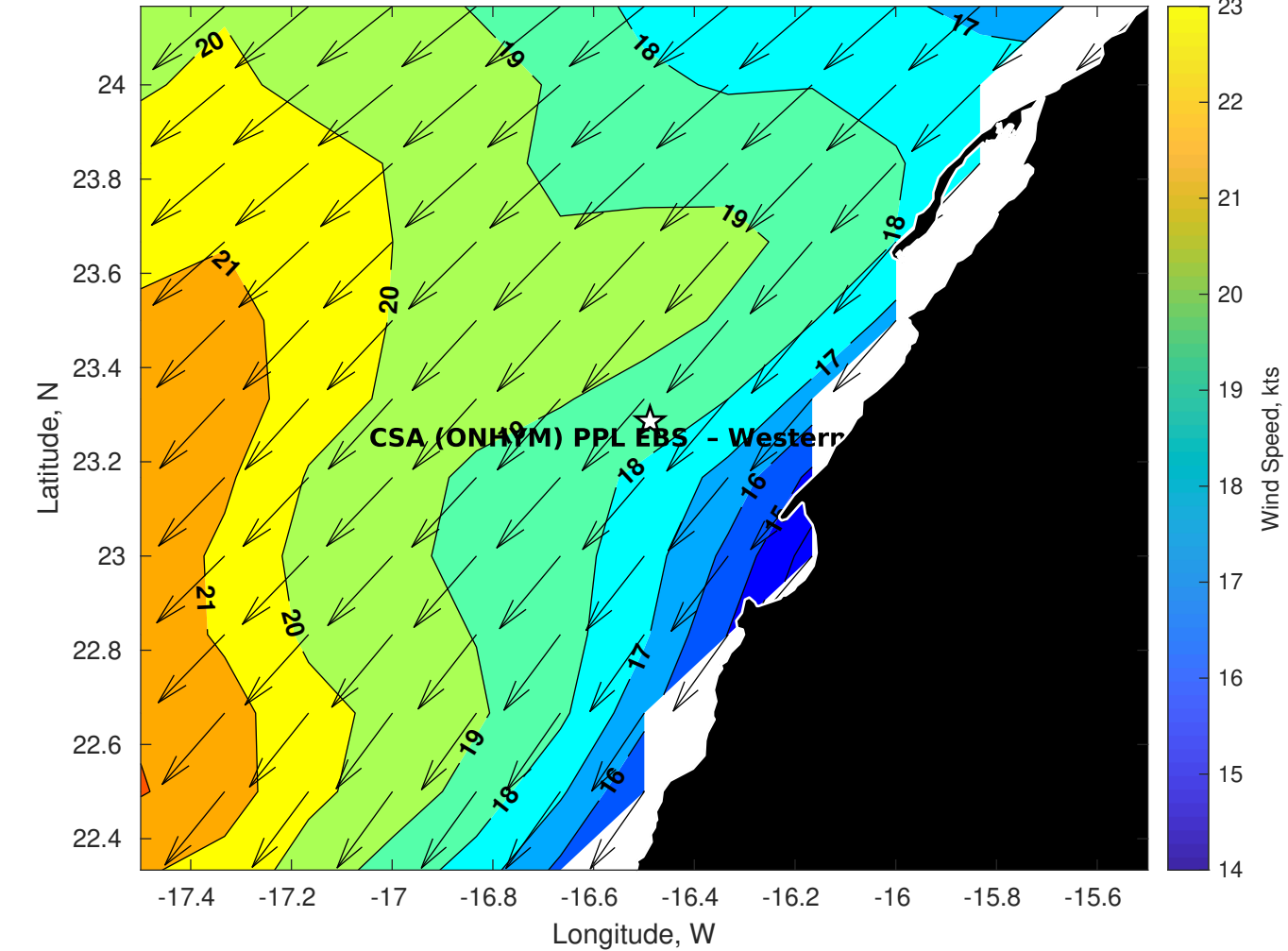
Winds (kts) for CSA (ONHYM) PPL EBS - Western Sahara at 08-Nov-2025 09:00:00
