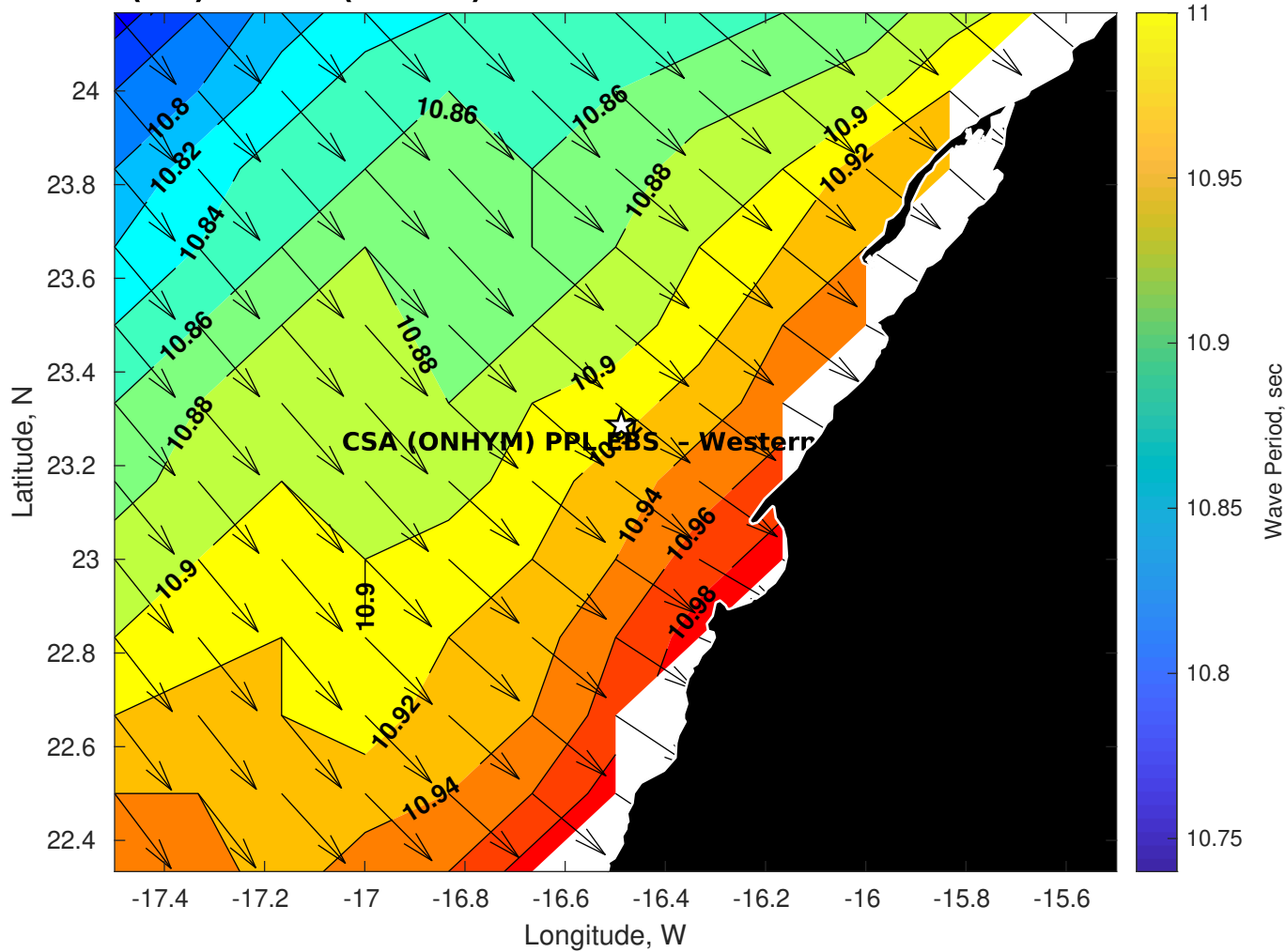
Wave Period (sec) for CSA (ONHYM) PPL EBS - Western Sahara at 08-Nov-2025 09:00:00
