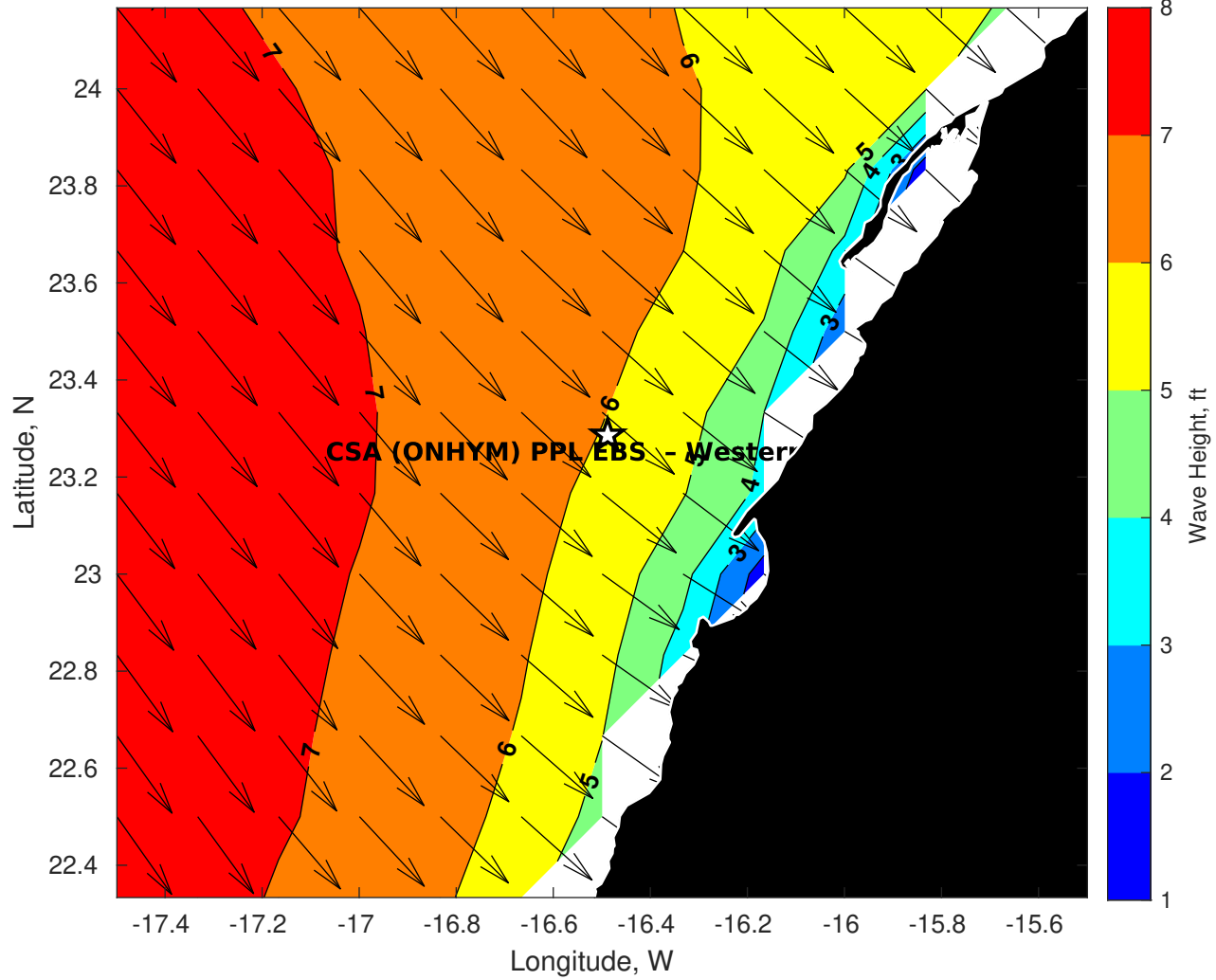
Wave Height (ft) for CSA (ONHYM) PPL EBS - Western Sahara at 08-Nov-2025 09:00:00
