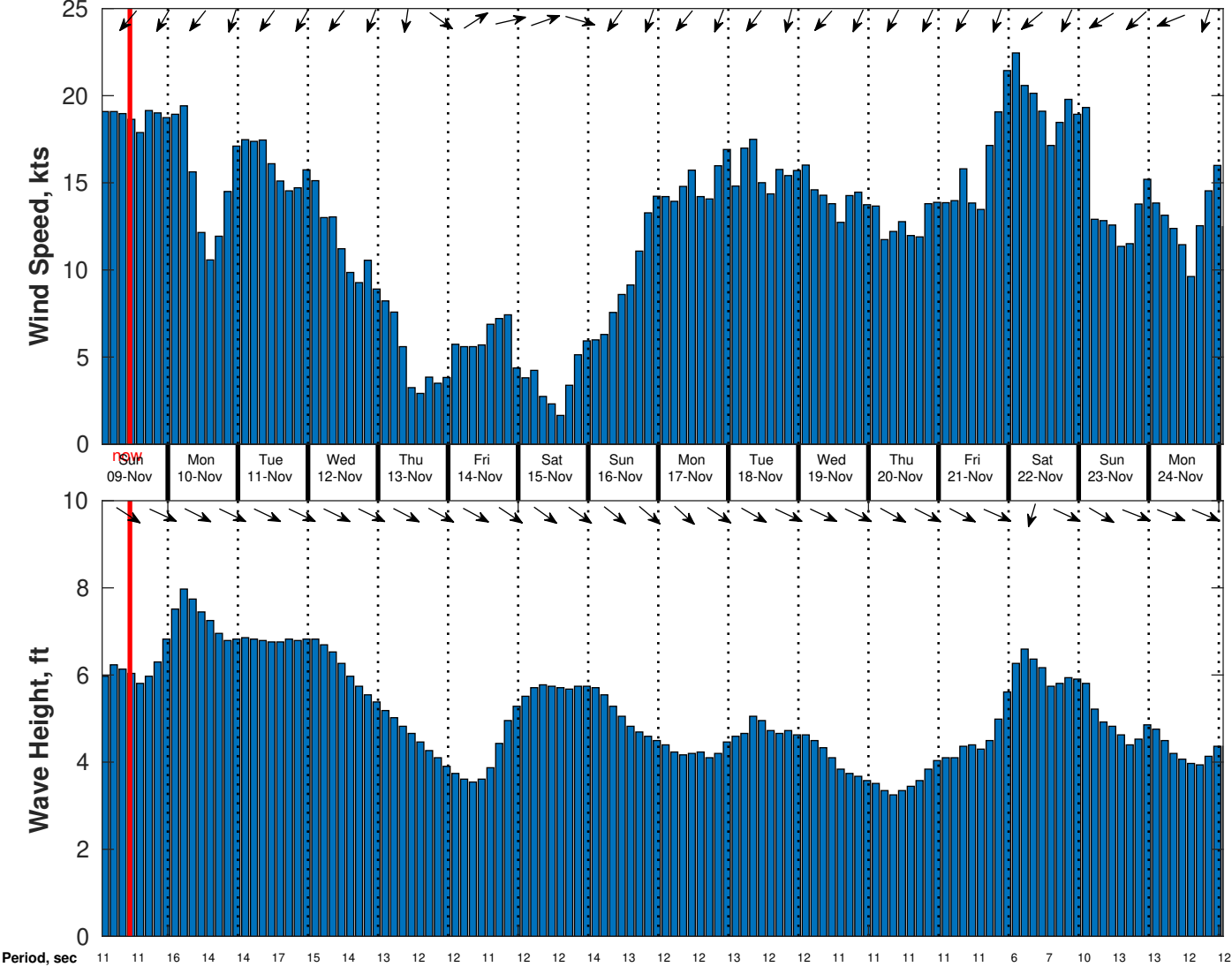
Wind & Wave Forecast for CSA (ONHYM) PPL EBS - Western Sahara from 08-Nov-2025 01:00:00 to 24-Nov-2025 01:00:00
