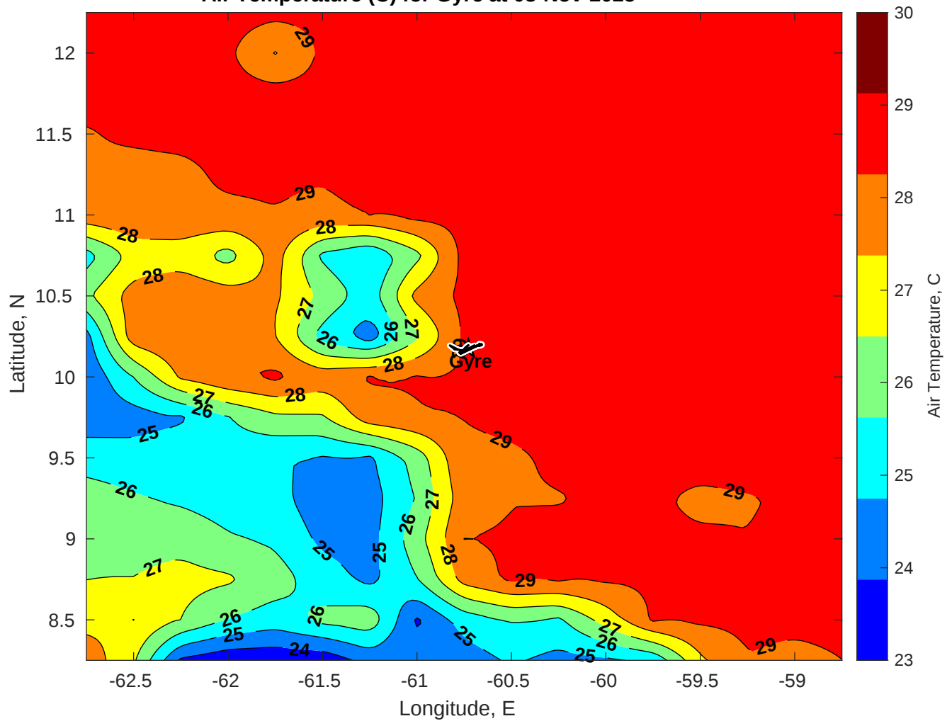
Air Temperature (C) for Gyre at 08-Nov-2025
