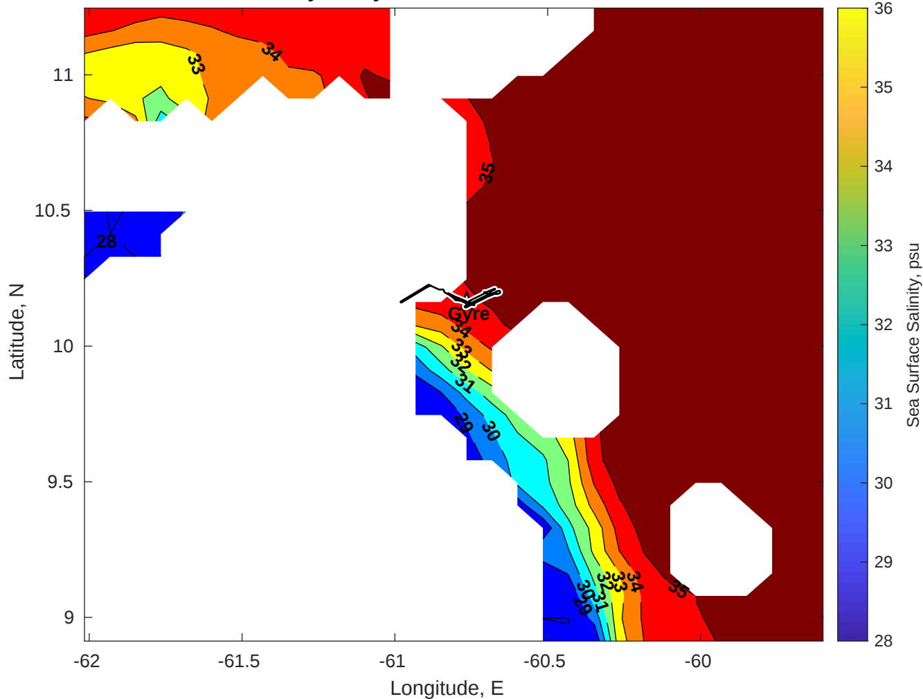
Surface Salinity for Gyre at 07-Nov-2025 00:00:00
