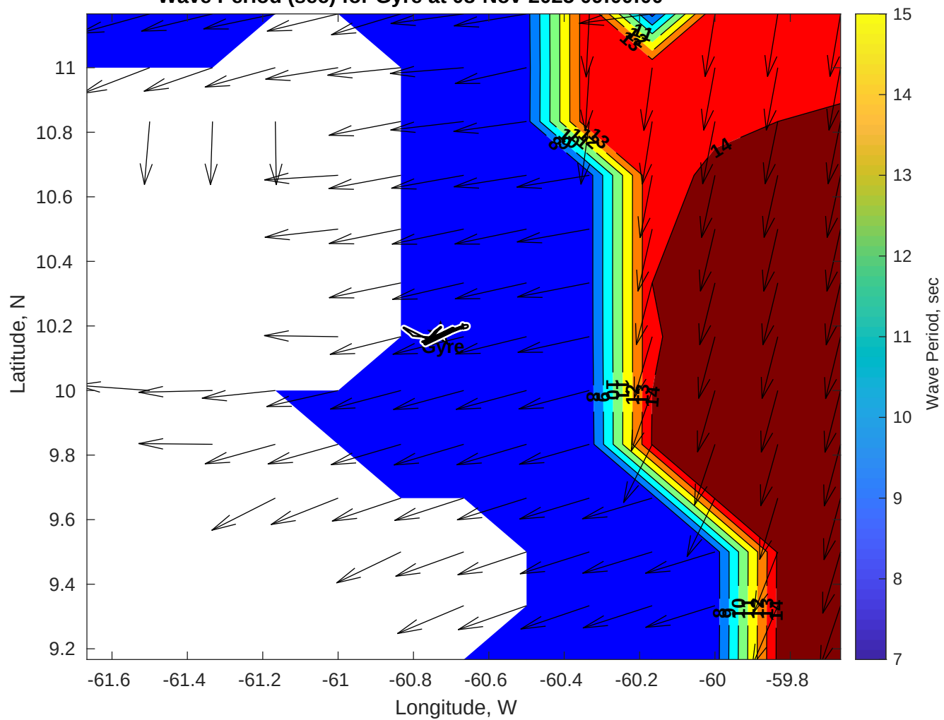
Wave Period (sec) for Gyre at 08-Nov-2025 09:00:00
