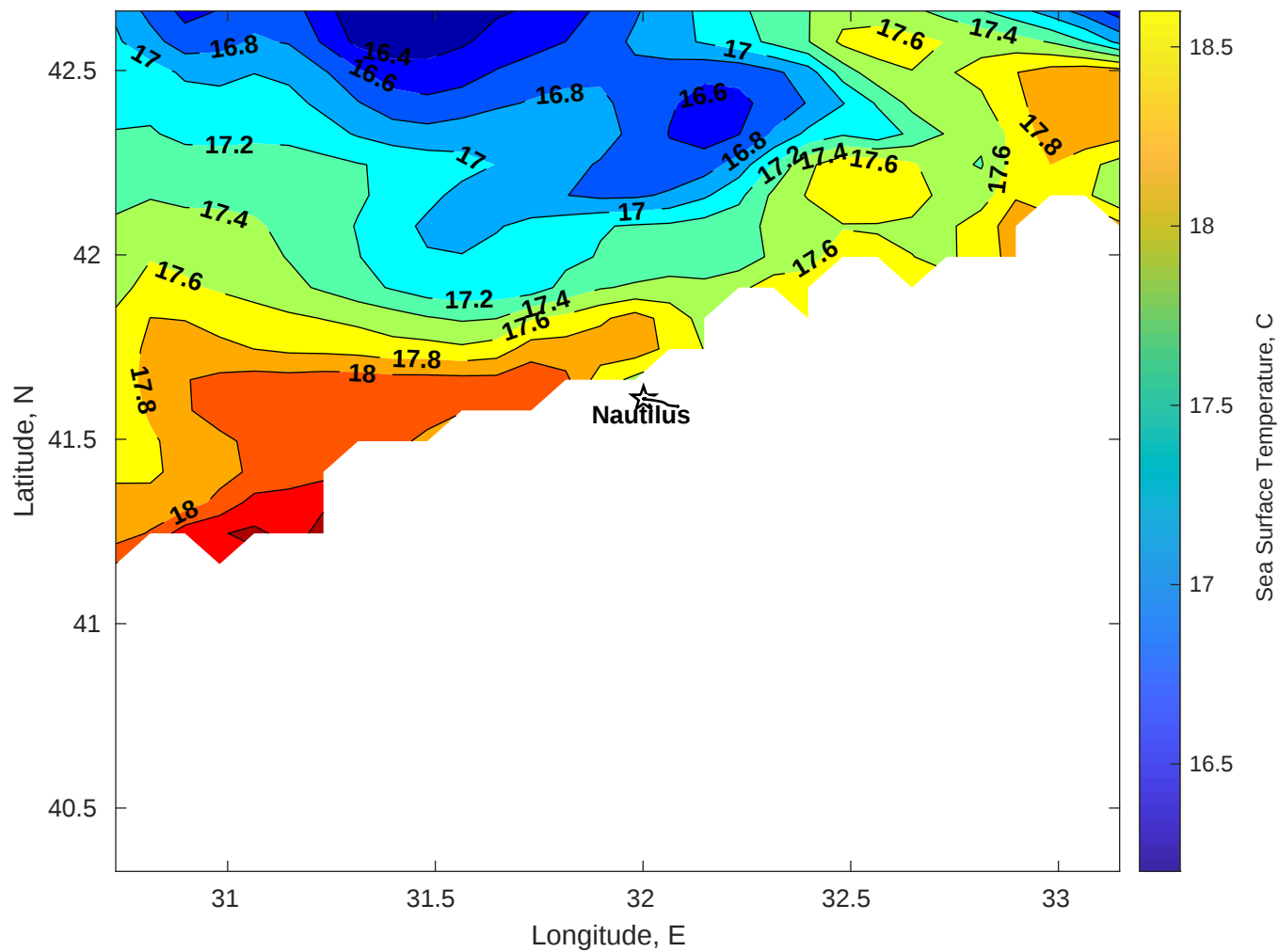
SST for Nautilus at 07-Nov-2025 00:00:00
