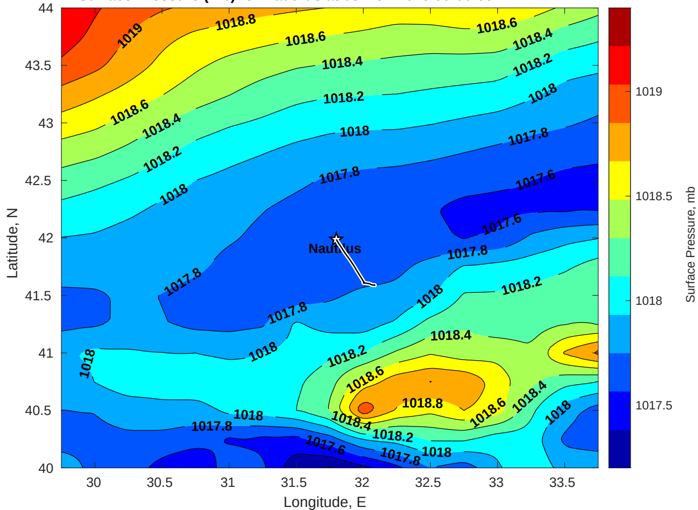
Surface Pressure (mb) for Nautilus at 08-Nov-2025 00:00:00
