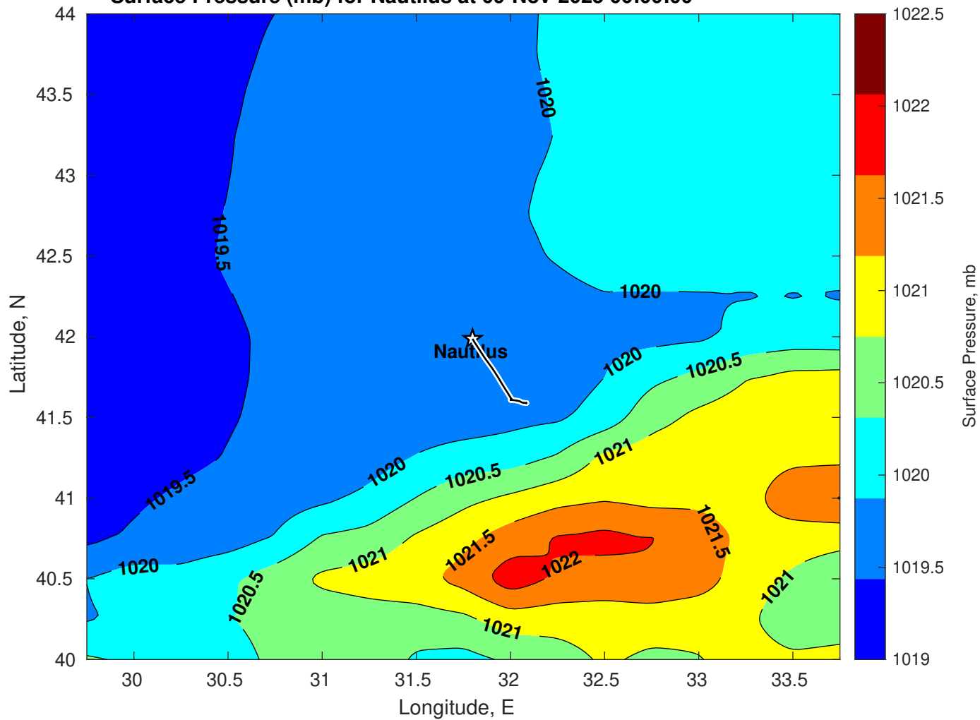
Surface Pressure (mb) for Nautilus at 09-Nov-2025 00:00:00
