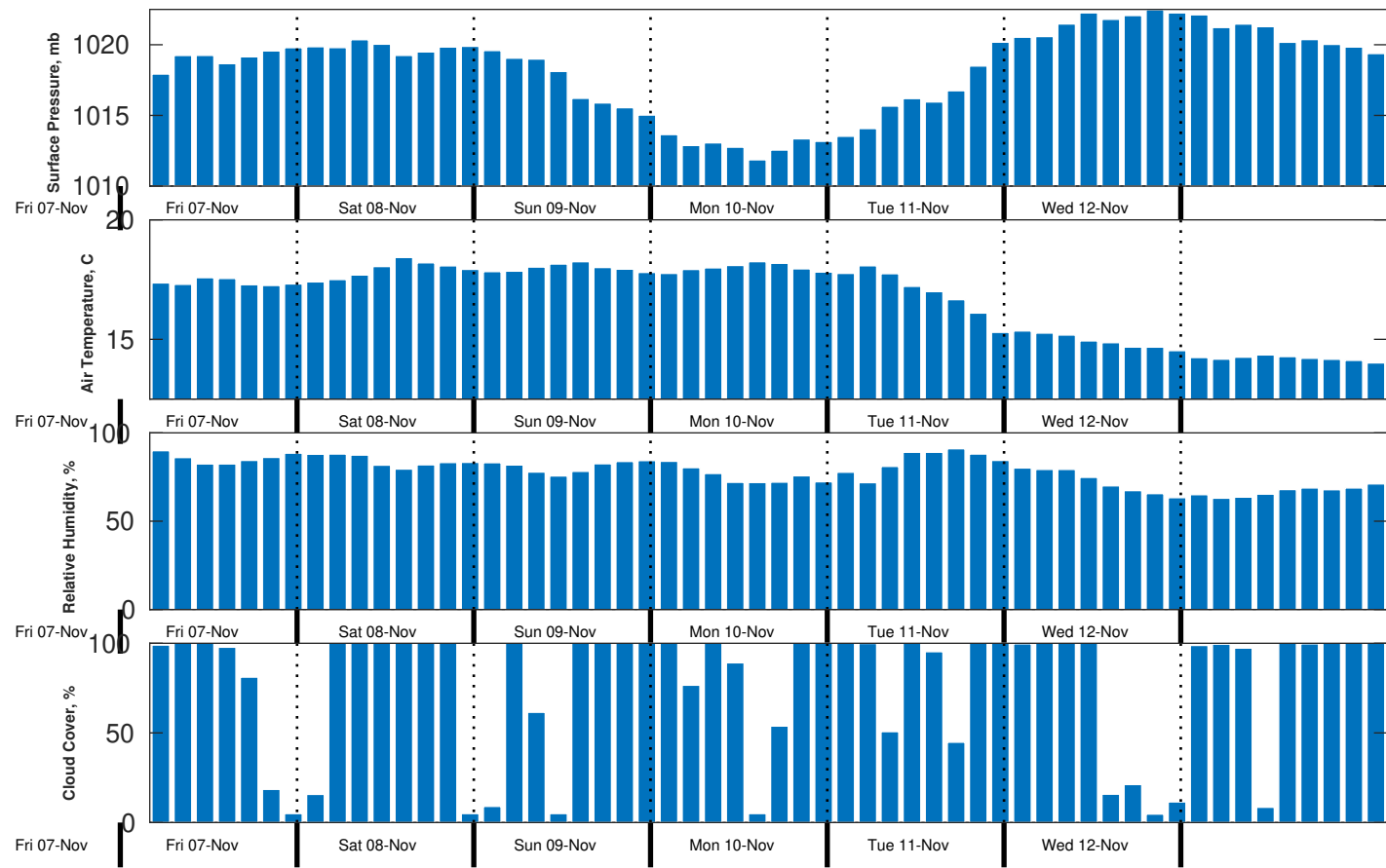
Met Forecast for Nautilus from 08-Nov-2025 00:00:00 to 15-Nov-2025 00:00:00
