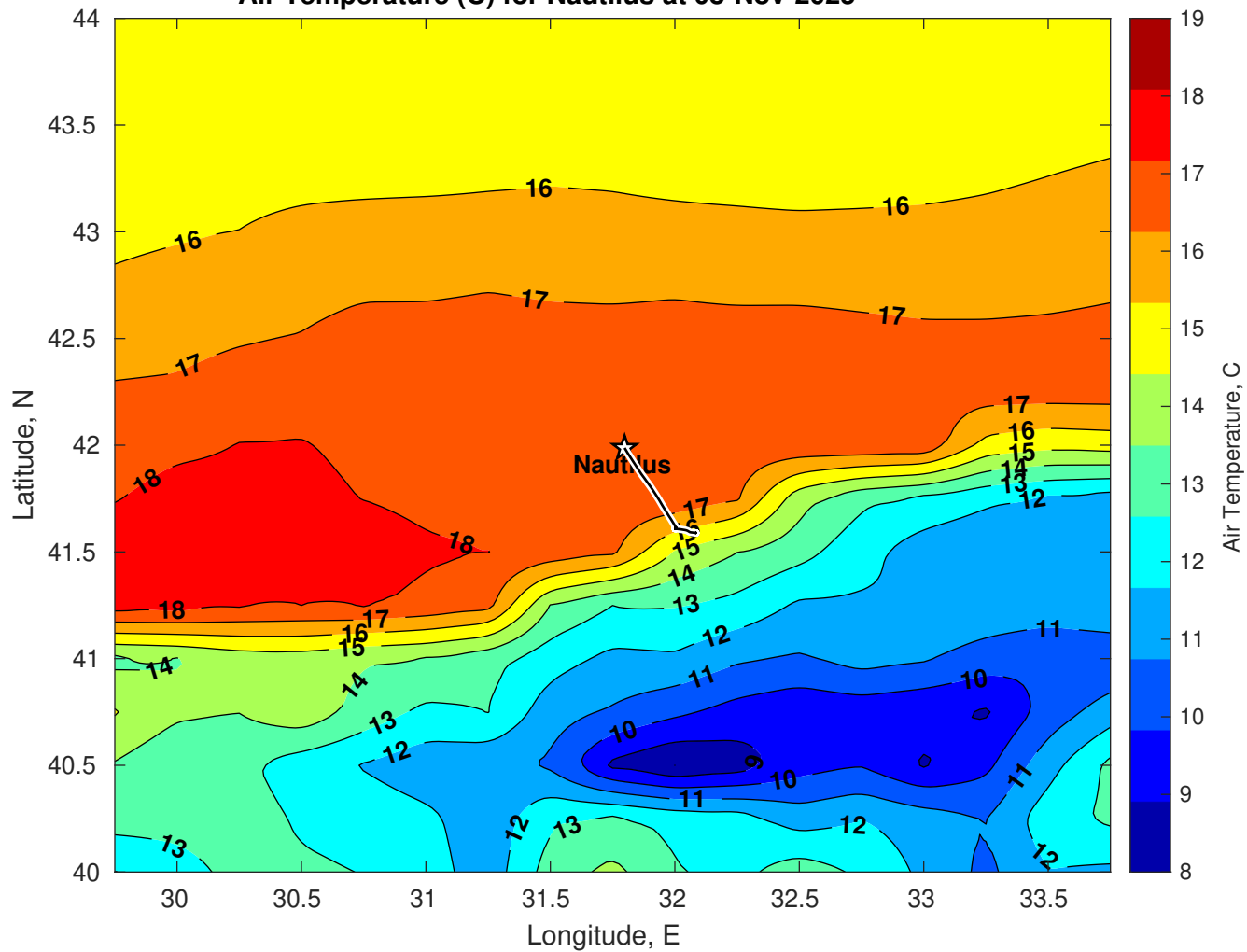
Air Temperature (C) for Nautilus at 08-Nov-2025
