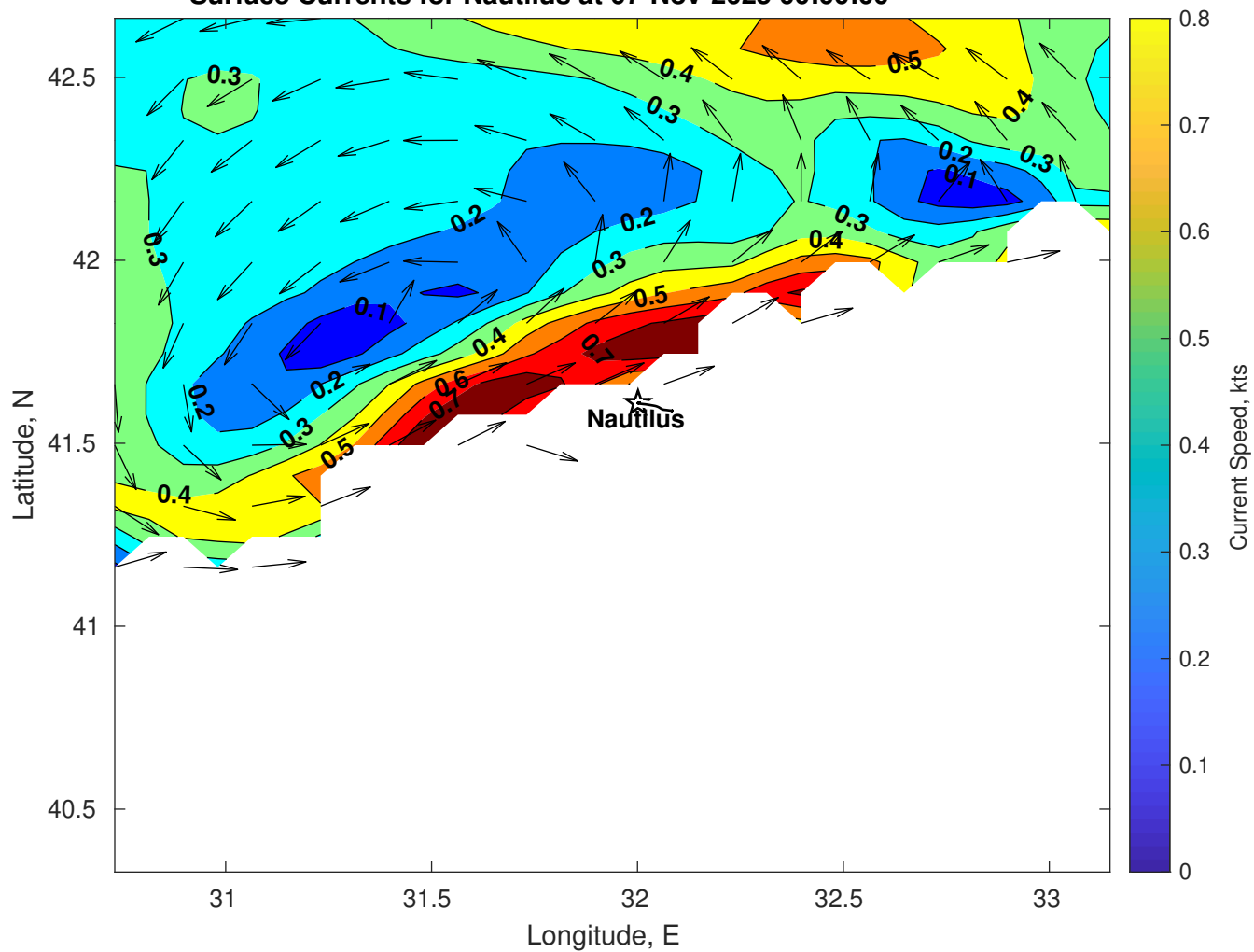
Surface Currents for Nautilus at 07-Nov-2025 00:00:00
