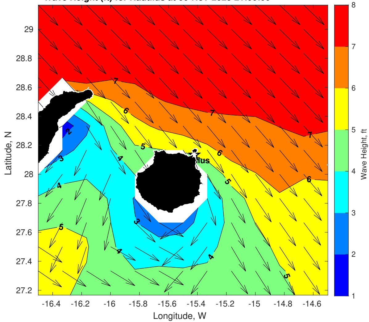
Wave Height (ft) for Nautilus at 06-Nov-2025 21:00:00
