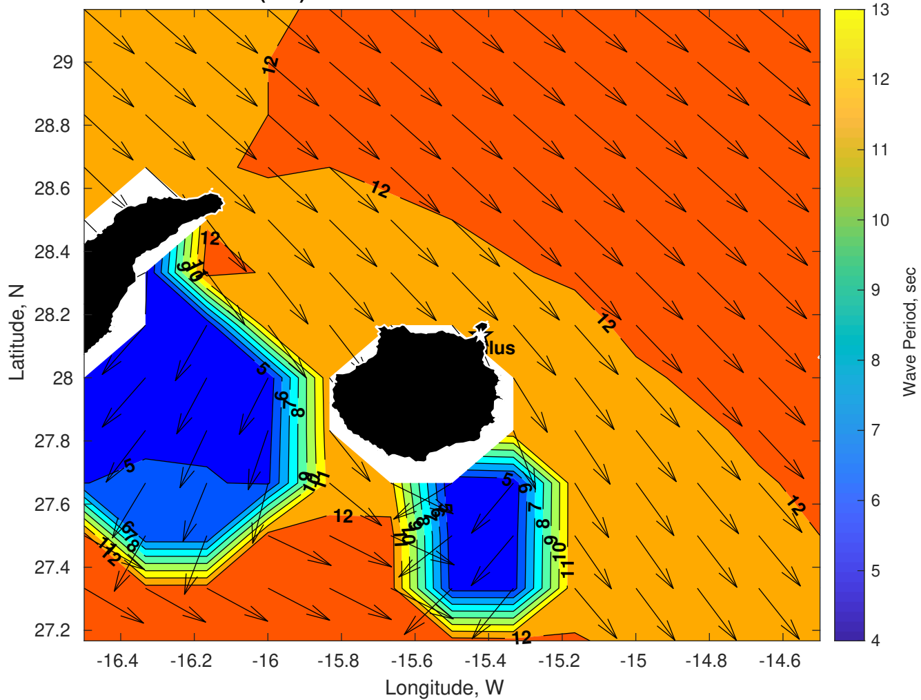
Wave Period (sec) for Nautilus at 06-Nov-2025 21:00:00
