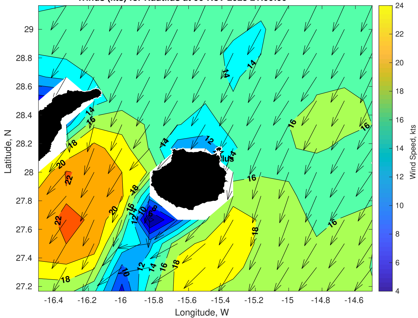
Winds (kts) for Nautilus at 06-Nov-2025 21:00:00
