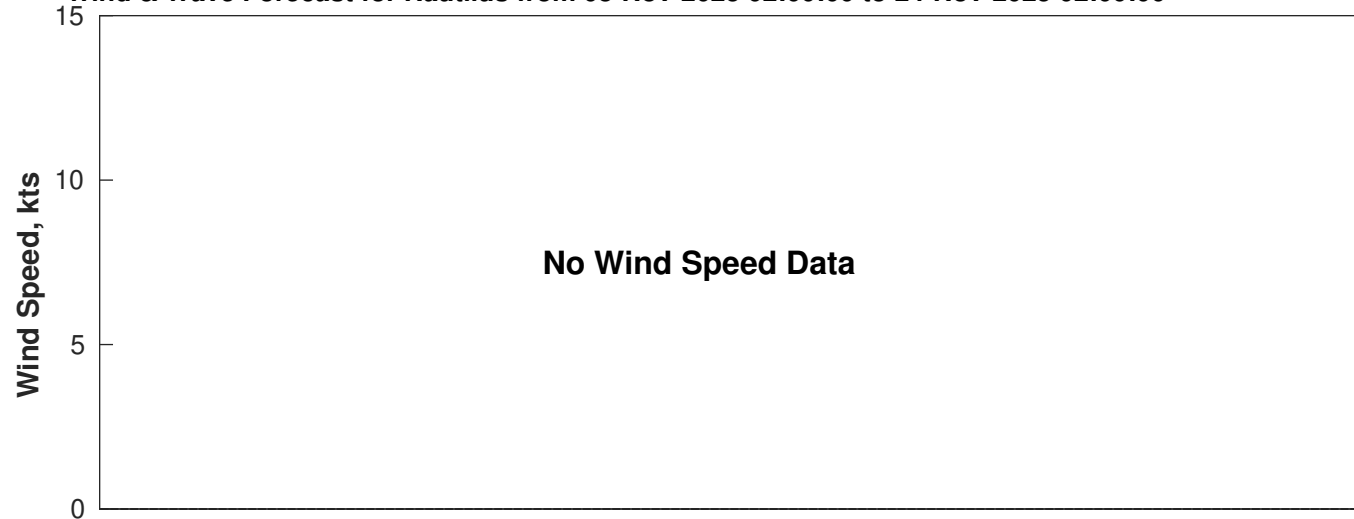
Wind & Wave Forecast for Nautilus from 08-Nov-2025 02:00:00 to 24-Nov-2025 02:00:00
