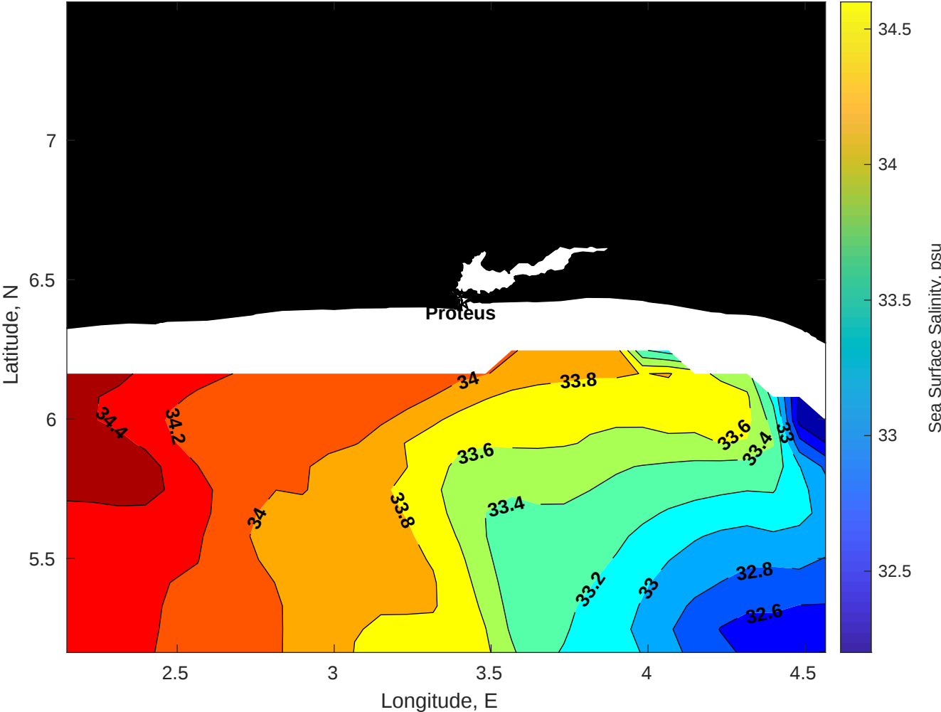
Surface Salinity for Proteus at 07-Nov-2025 00:00:00
