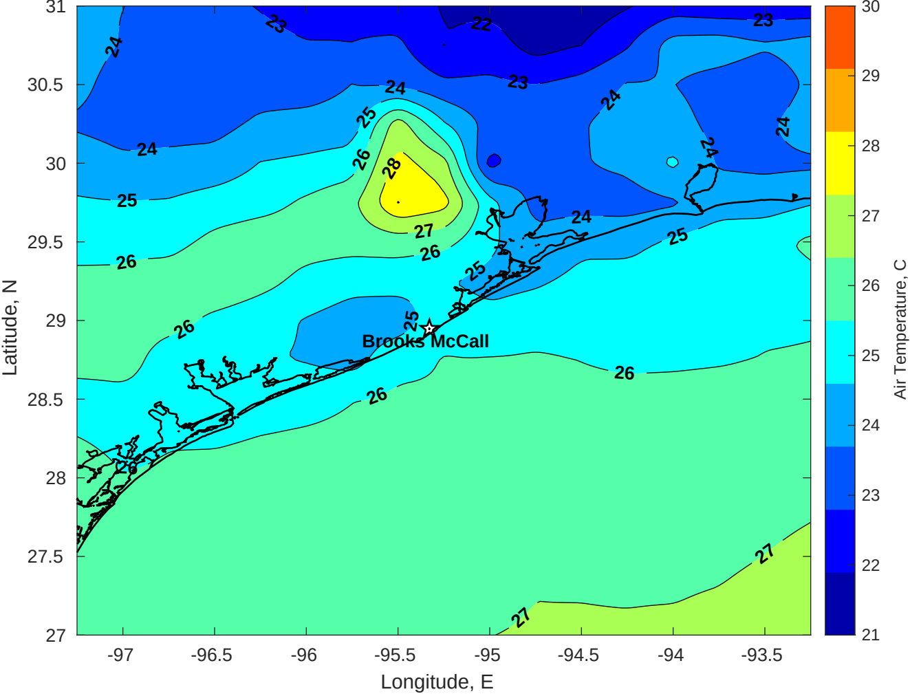
Air Temperature (C) for Brooks McCall at 09-Nov-2025
