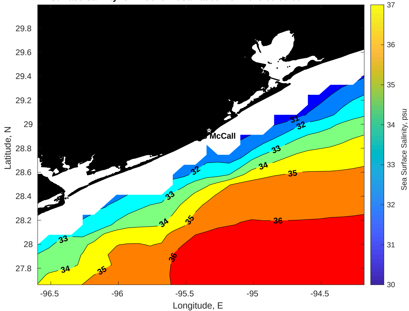
Surface Salinity for Brooks McCall at 08-Nov-2025 00:00:00
