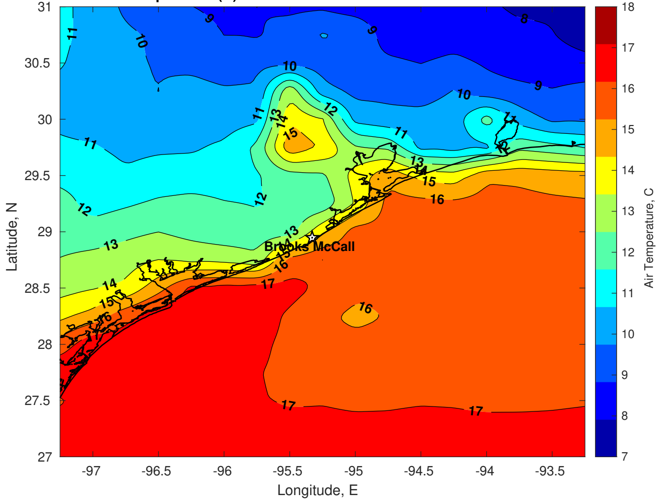
Air Temperature (C) for Brooks McCall at 09-Nov-2025
