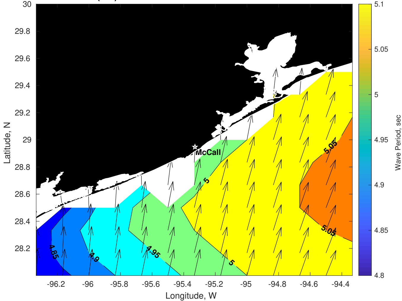
Wave Period (sec) for Brooks McCall at 09-Nov-2025 09:00:00
