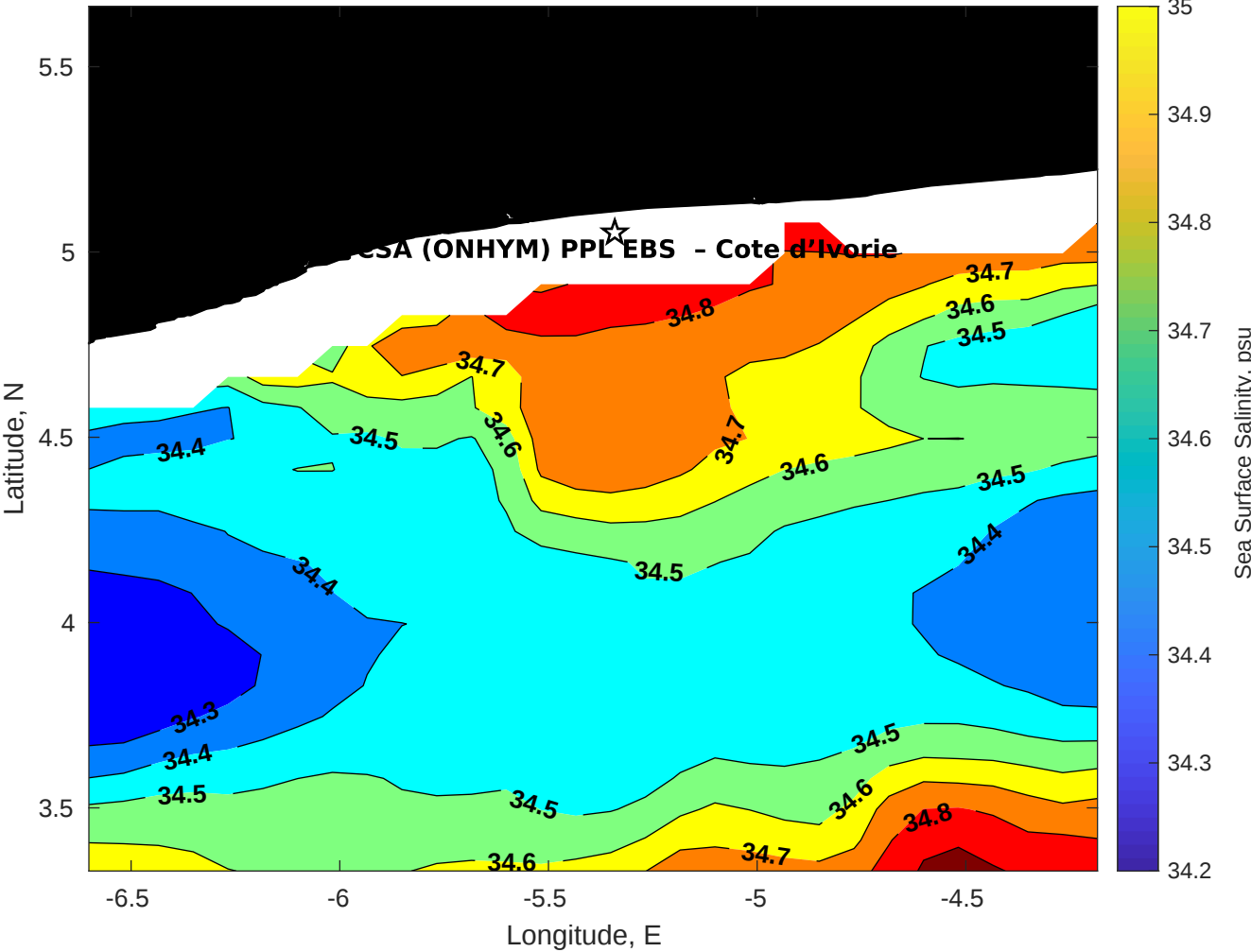
Surface Salinity for CSA (ONHYM) PPL EBS - Cote d'Ivoire at 08-Nov-2025 00:00:00
