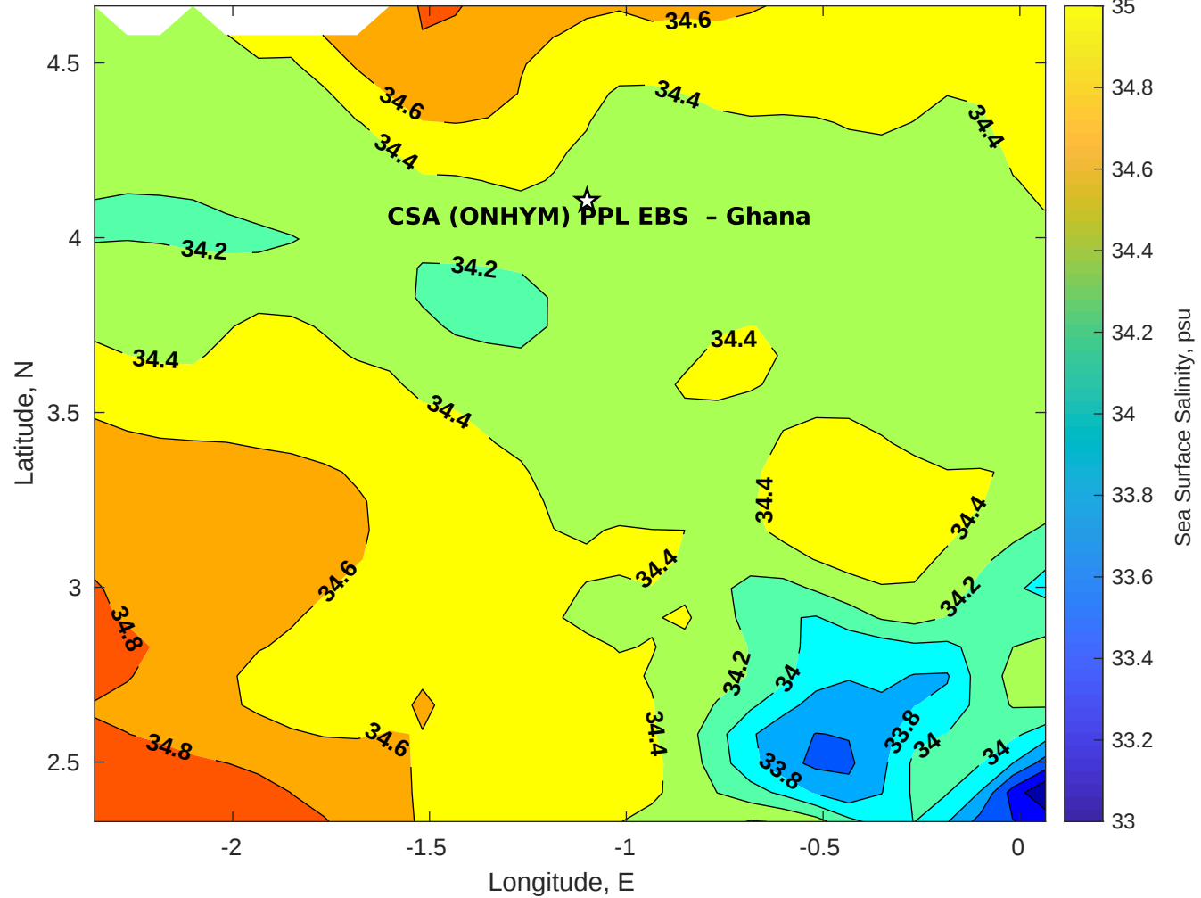
Surface Salinity for CSA (ONHYM) PPL EBS - Ghana at 08-Nov-2025 00:00:00
