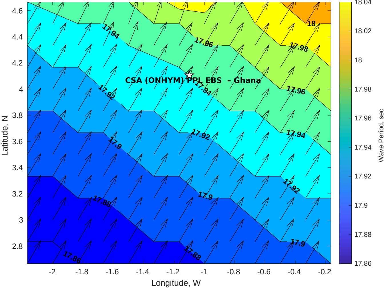
Wave Period (sec) for CSA (ONHYM) PPL EBS - Ghana at 09-Nov-2025 09:00:00
