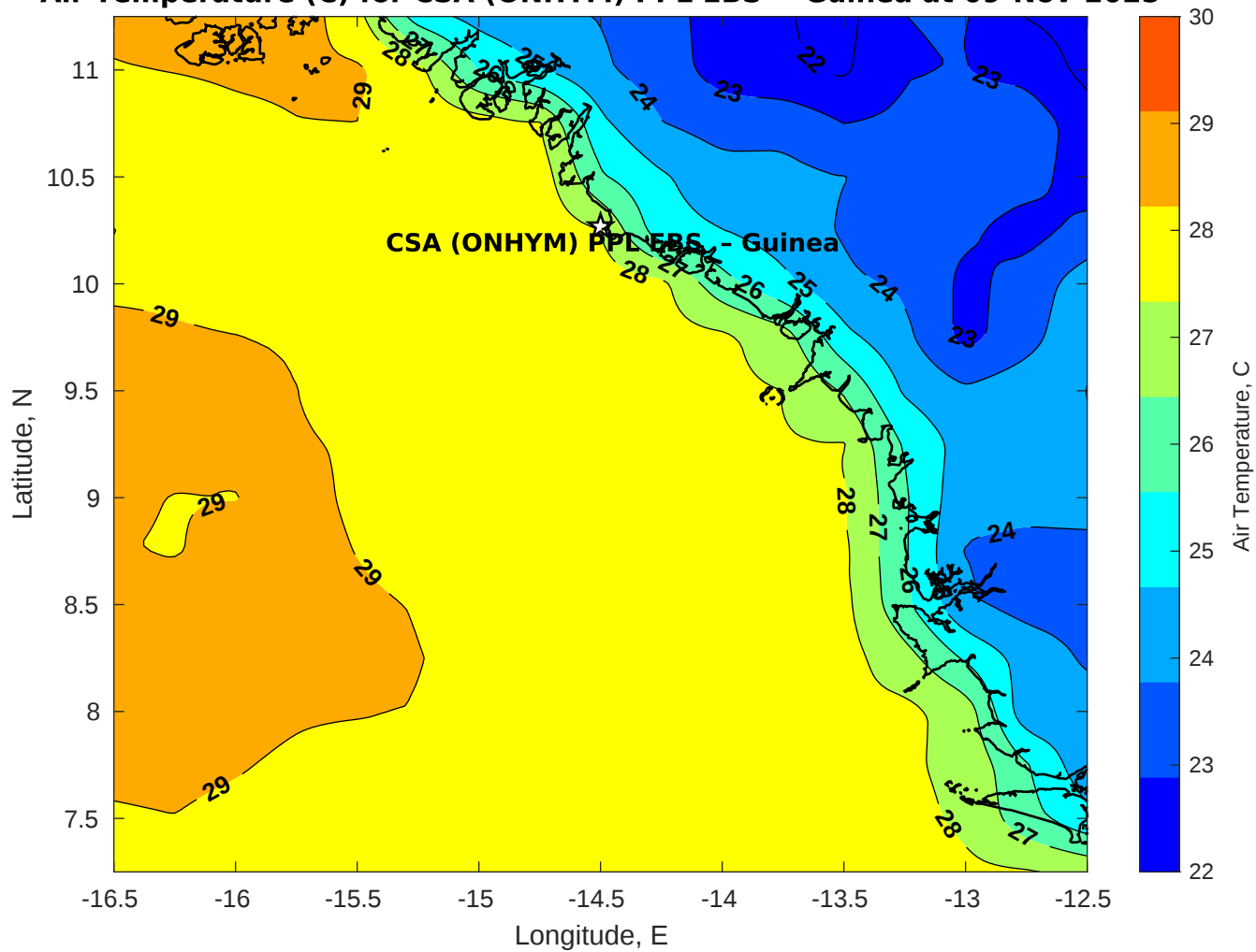
Air Temperature (C) for CSA (ONHYM) PPL EBS - Guinea at 09-Nov-2025
