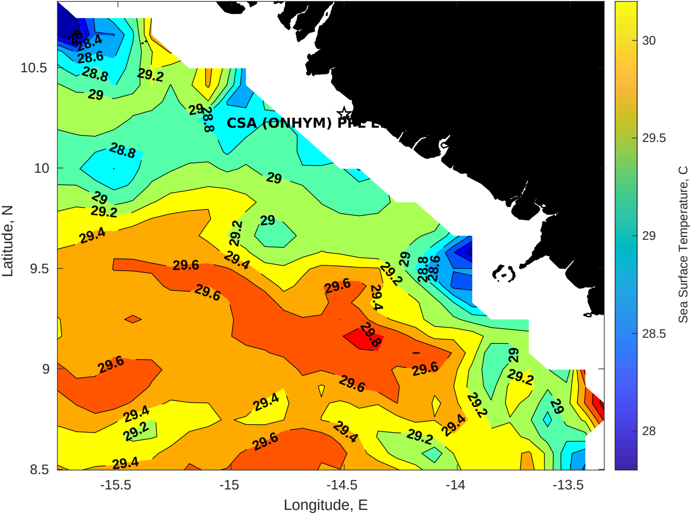
SST for CSA (ONHYM) PPL EBS - Guinea at 08-Nov-2025 00:00:00
