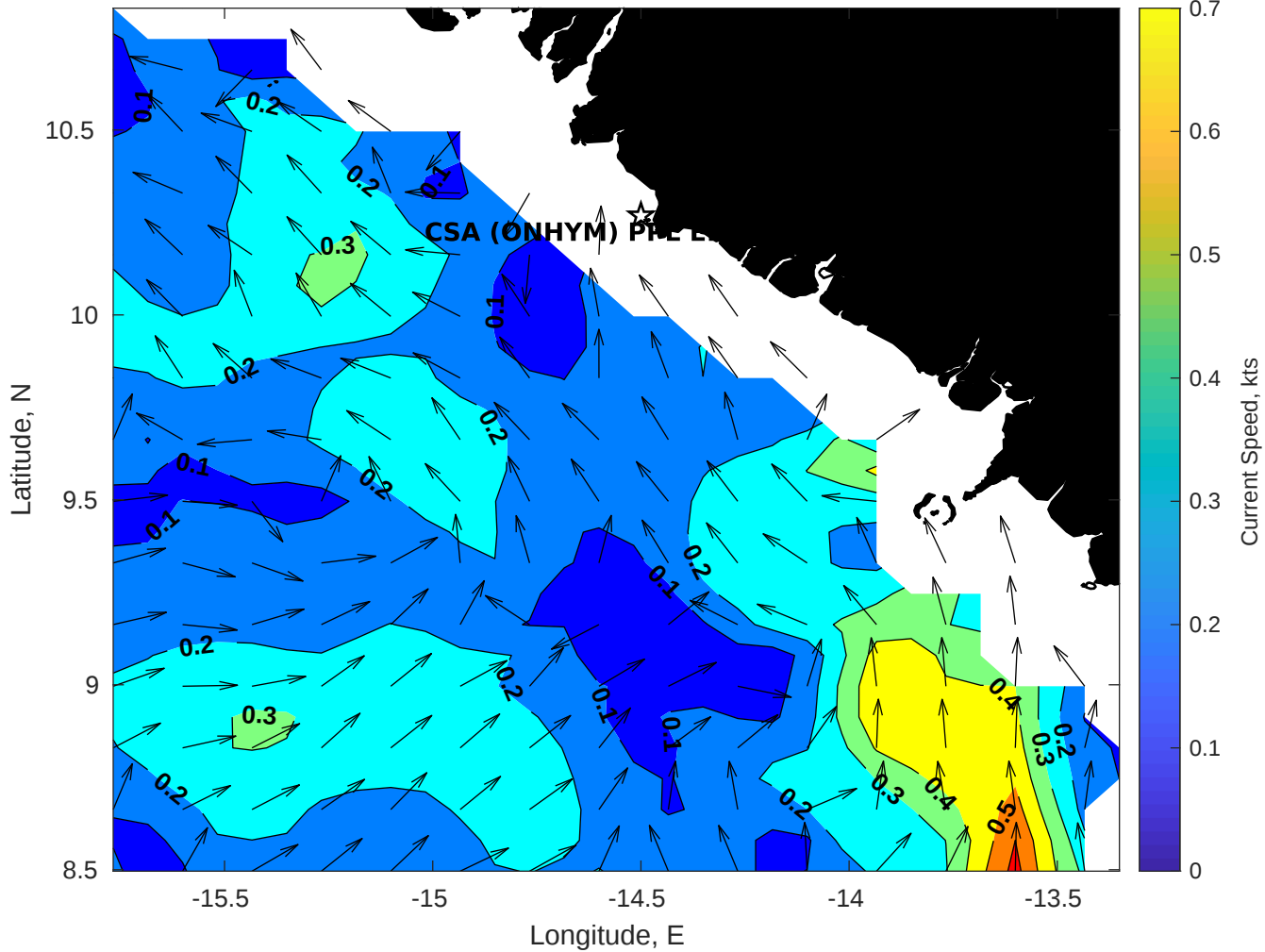
Surface Currents for CSA (ONHYM) PPL EBS - Guinea at 08-Nov-2025 00:00:00
