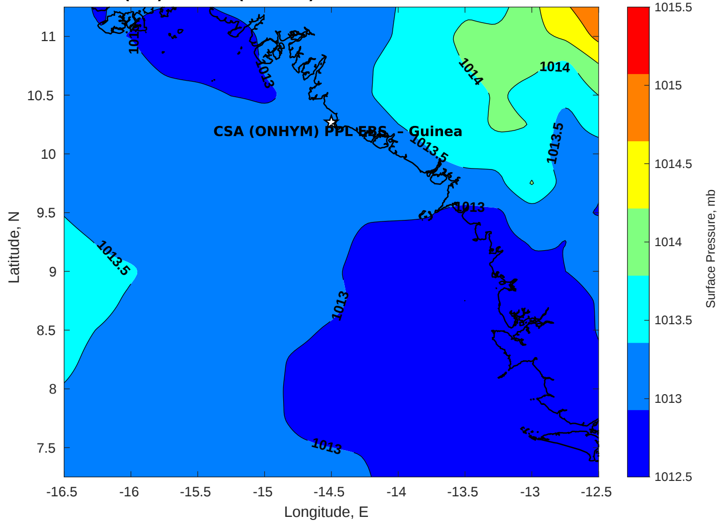
Surface Pressure (mb) for CSA (ONHYM) PPL EBS - Guinea at 11-Nov-2025 00:00:00
