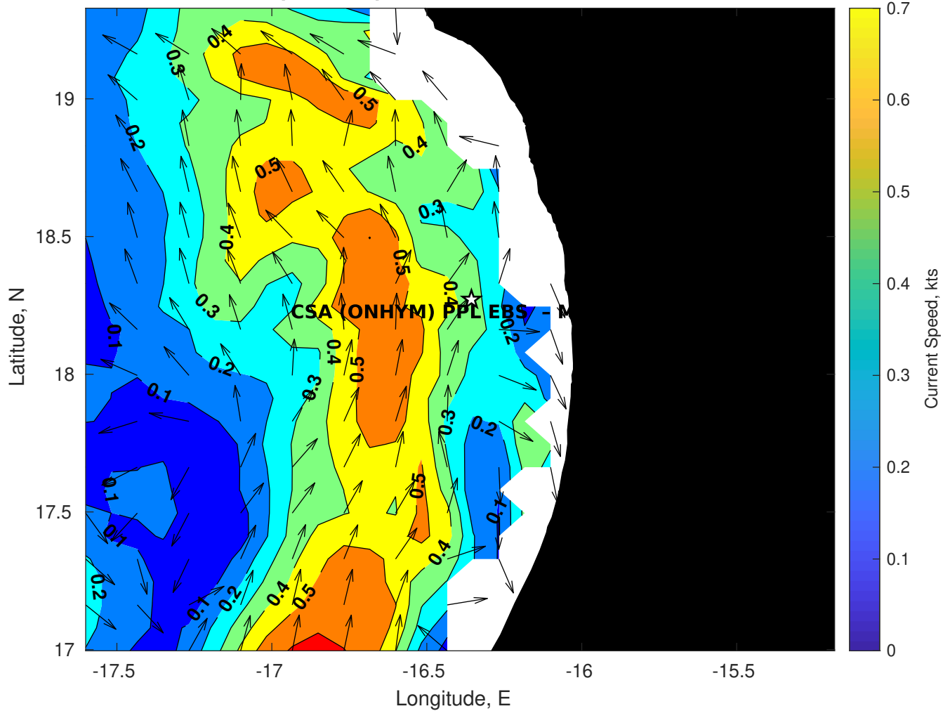
Surface Currents for CSA (ONHYM) PPL EBS - Mauritania at 08-Nov-2025 00:00:00
