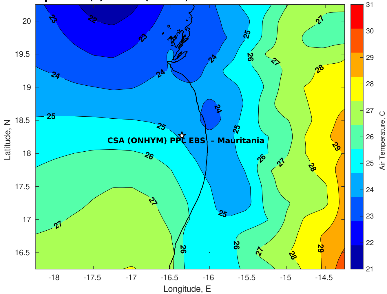
Air Temperature (C) for CSA (ONHYM) PPL EBS - Mauritania at 09-Nov-2025
