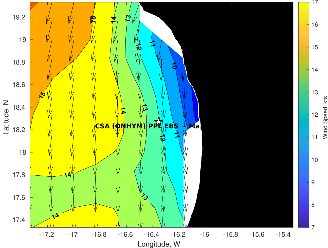
Winds (kts) for CSA (ONHYM) PPL EBS - Mauritania at 09-Nov-2025 09:00:00
