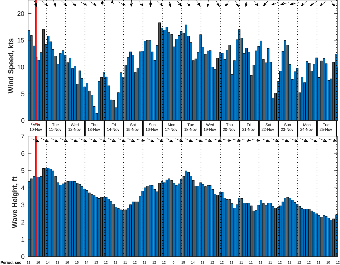
Wind & Wave Forecast for CSA (ONHYM) PPL EBS - Mauritania from 09-Nov-2025 01:00:00 to 25-Nov-2025 01:00:00
